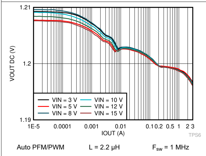
Figure 8-76. Output Voltage vs Output Current V OUT = 1.2 V
