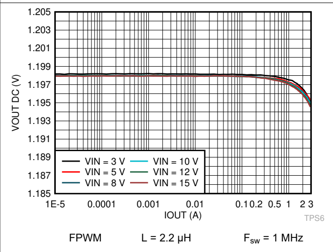
Figure 8-77. Output Voltage vs Output Current V OUT = 1.2 V
