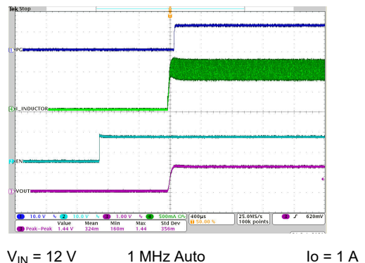
V IN = 12 V 1 MHz Auto PFM/PWM I o = 1 A V OUT = 1.2 V T A = 25°C
