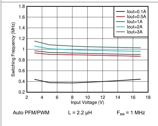
Figure 8-33. Switching Frequency vs Input Voltage V_{OUT} = 1.2\text{ V}
