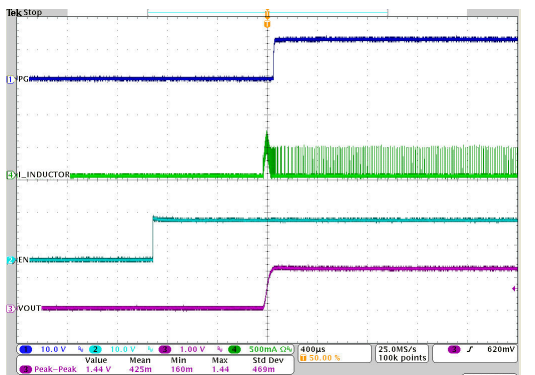
V IN = 12 V 1 MHz Auto PFM/PWM I o = 10 mA V OUT = 1.2 V T A = 25°C
