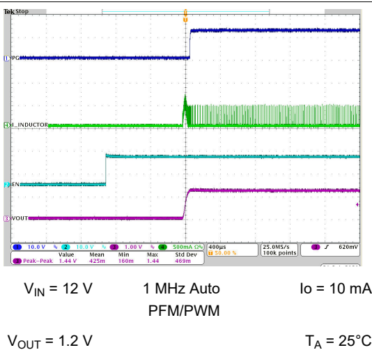
Figure 8-39. Start-up Timing
