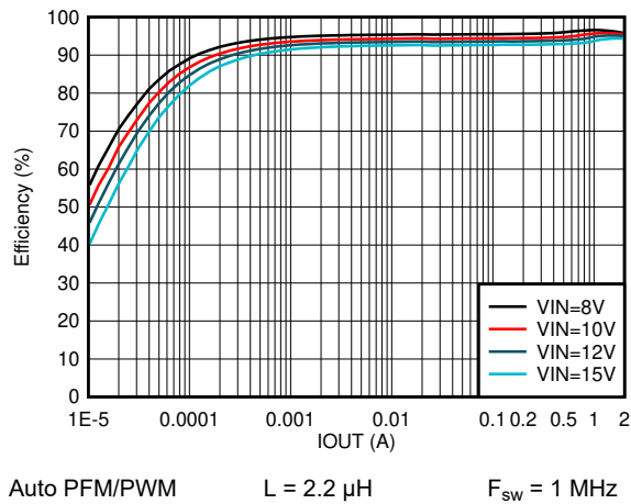
Figure 8-5. Efficiency vs Output Current V OUT = 5 V
