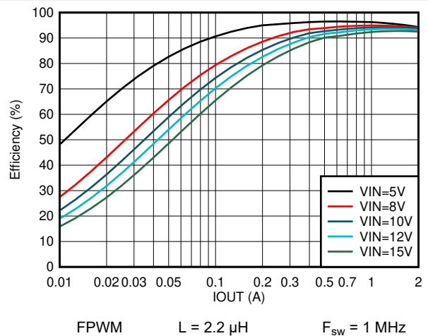
Figure 8-8. Efficiency vs Output Current V OUT = 5 V
