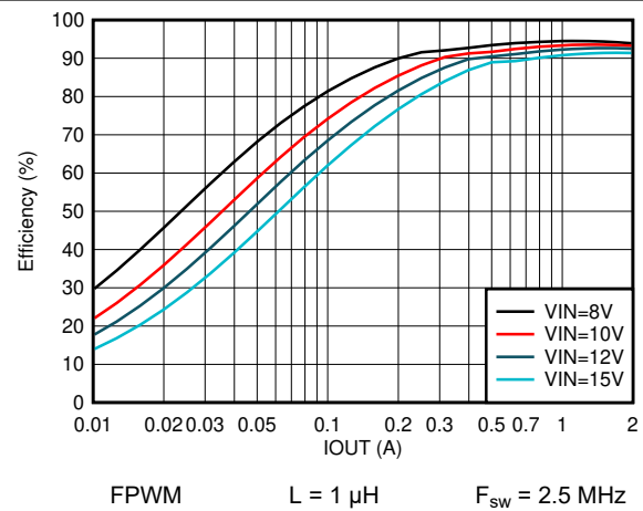
Figure 8-6. Efficiency vs Output Current V OUT = 5 V
