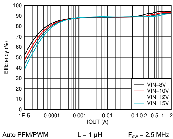
Figure 8-5. Efficiency vs Output Current V OUT = 5 V
