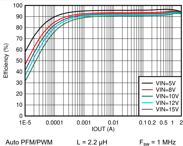
Figure 8-7. Efficiency vs Output Current V OUT = 5 V
