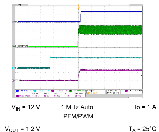
Figure 8-40. Start-up Timing
