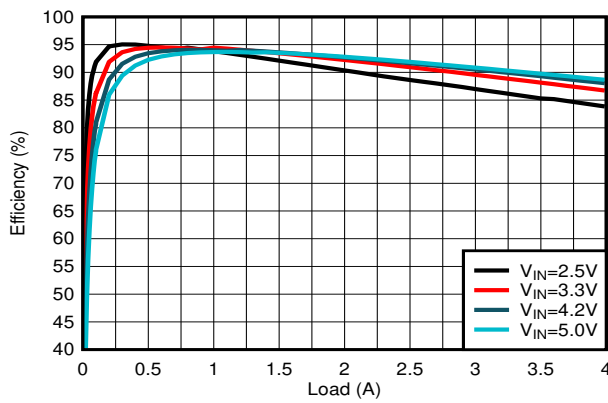
Figure 9-11. Efficiency
