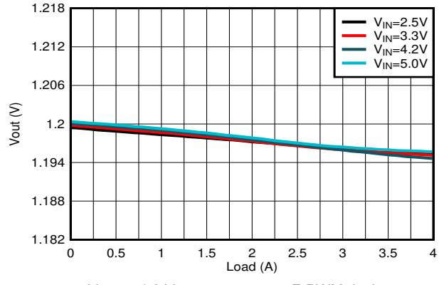
Figure 9-10. Load Regulation
