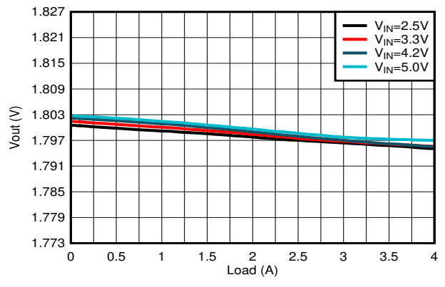
Figure 9-14. Load Regulation
