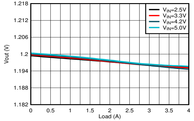
V OUT = 1.2 V F-PWM devices
