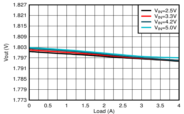
V OUT = 1.8 V F-PWM devices
