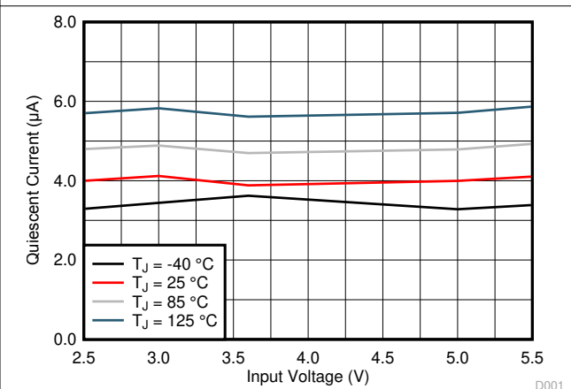
Figure 7-4. Quiescent Current
