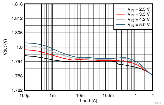
V OUT = 1.8 V
