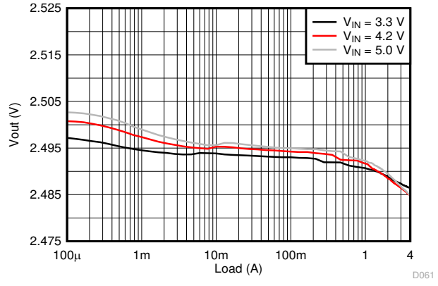
Figure 9-16. Load Regulation
