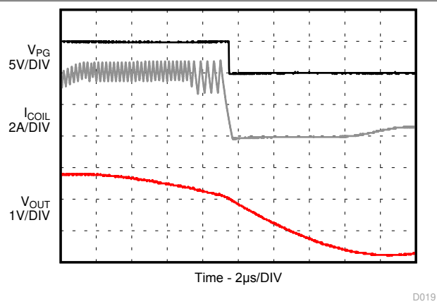
I OUT = 1 A TPS6282x
