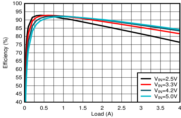
V OUT = 1.2 V F-PWM devices
