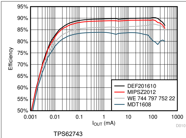
Figure 9-8. Efficiency vs Load Current; V_{OUT} = 1.8\text{ V}
