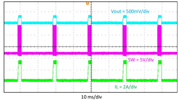
Figure 9-15. Hiccup, I_{out} = 5\text{ A}
