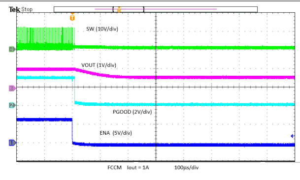
Figure 8-15. Prebias Power-Down
