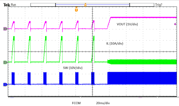
Figure 8-30. Hiccup Overcurrent
