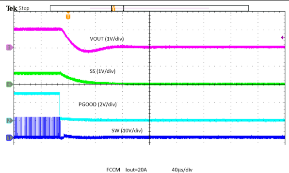
Figure 8-27. Over Temperature Protection in FCCM
