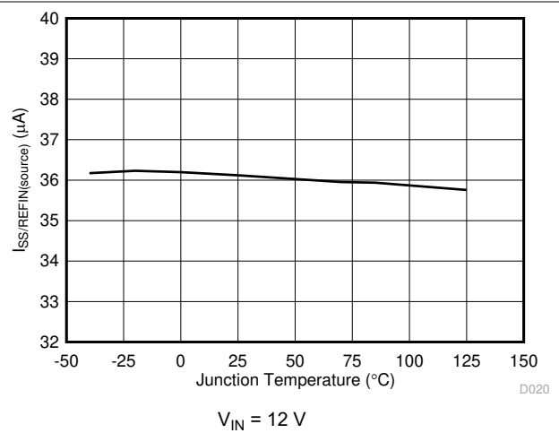
Figure 6-14. I SS(source) vs Junction Temperature
