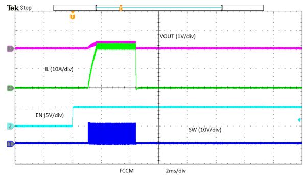
Figure 8-29. Enabled into Overcurrent
