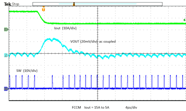
Figure 8-21. Unload Transient
