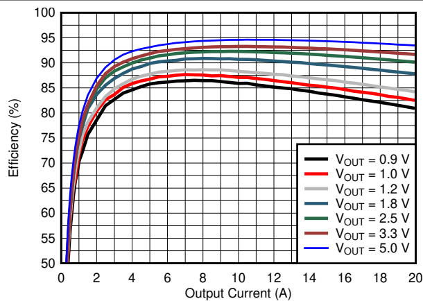
Figure 6-3. Efficiency vs Output Current, 12 V_{IN} , 800 KHz, FCCM, V_{CC} = \text{Int}
