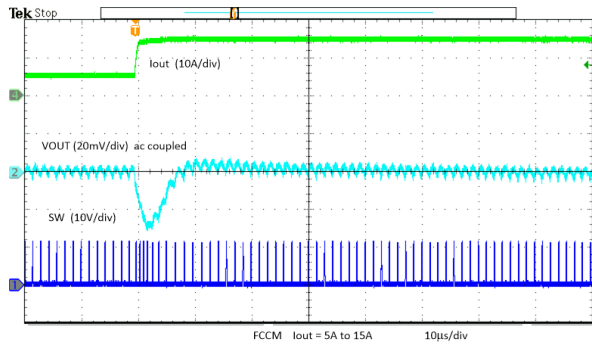
Figure 8-20. Load Transient
