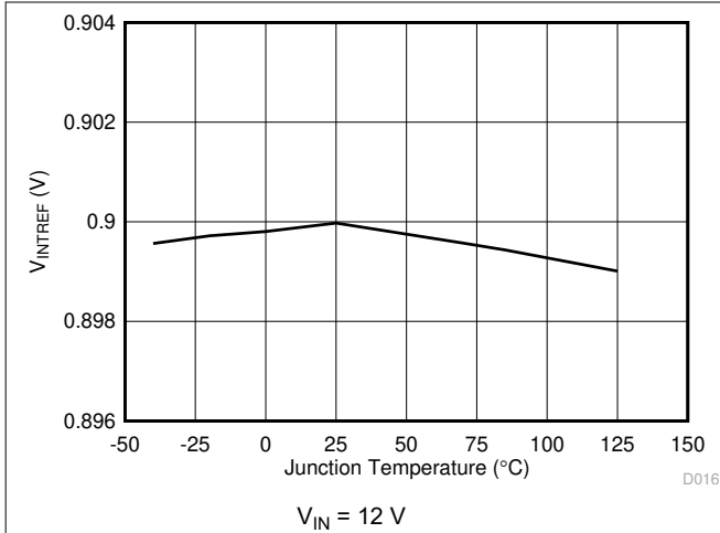
Figure 6-13. V INTREF vs Junction Temperature
