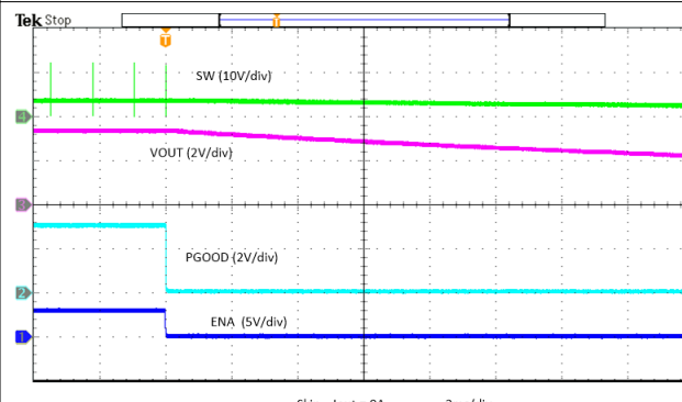
Figure 8-15. Prebias Power-Down
