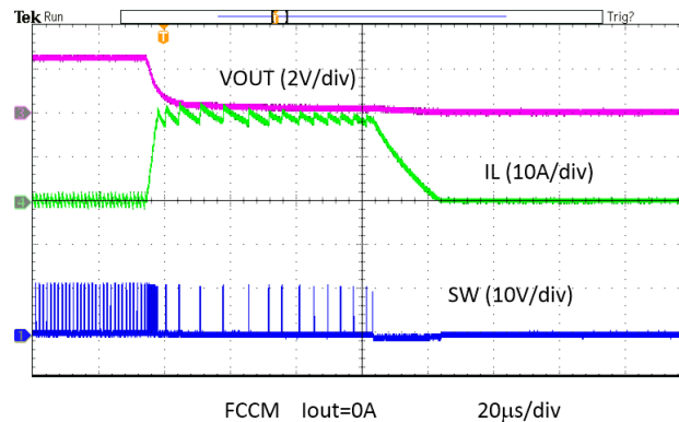
Figure 7-4. Overcurrent Protection
