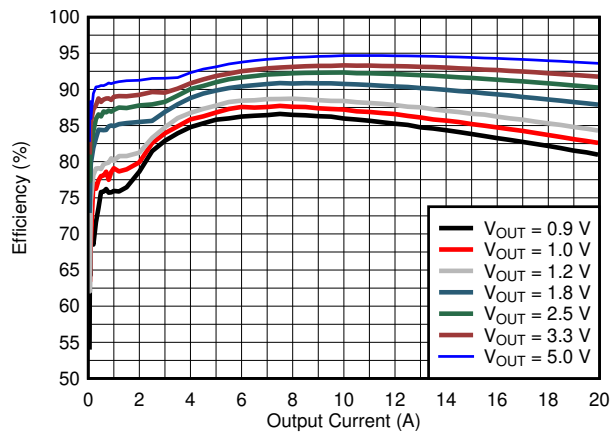
Figure 6-1. Efficiency vs Output Current, 12 V_{IN} , 800 KHz, DCM, V_{CC} = \text{Int}
