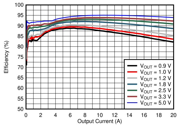
Figure 6-2. Efficiency vs Output Current, 12 V_{IN} , 800 KHz, DCM, V_{CC} = \text{EXT } 3.3 \text{ V}
