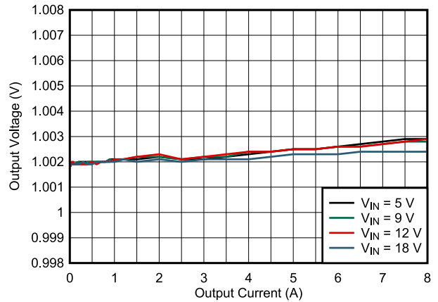
Figure 8-5. Load Regulation
