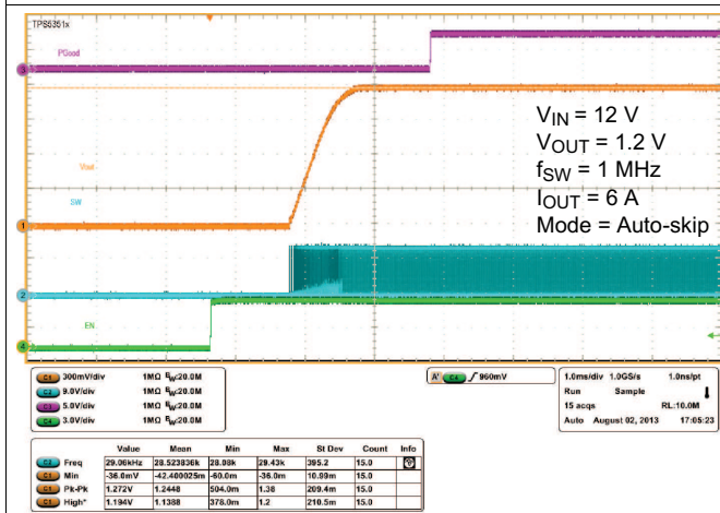
Figure 21. Auto-Skip Mode Start-Up
