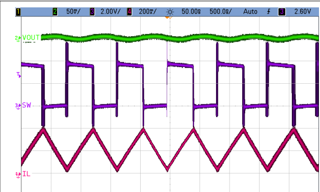
Figure 9-9. PWM Mode Operation
