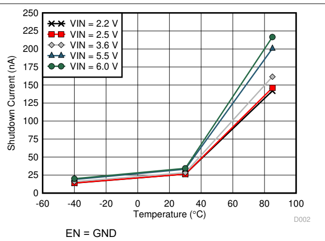
Figure 7-2. Shutdown Current I_{SD} vs Temperature
