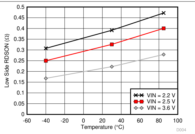
Figure 7-4. Low-side R_{DS(on)} vs Temperature
