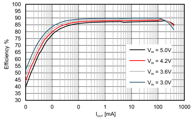
Figure 9-3. Efficiency vs Load Current; V_{OUT} = 1.8\text{ V}
