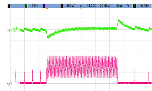
Figure 9-13. Load Transient Response; 5 mA to 290 mA
