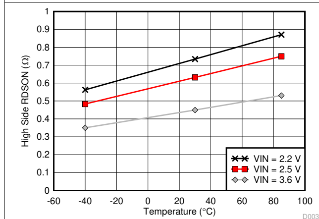
Figure 7-3. High Side R_{DS(on)} vs Temperature
