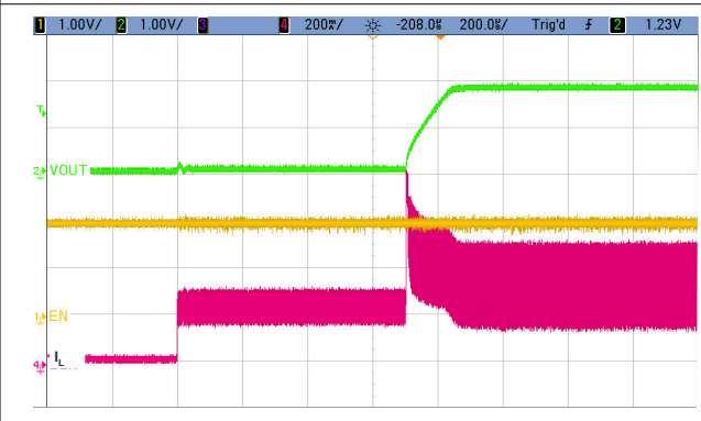
Figure 9-11. Startup Into 300 mA Electronic Load Soft-Start Delay
