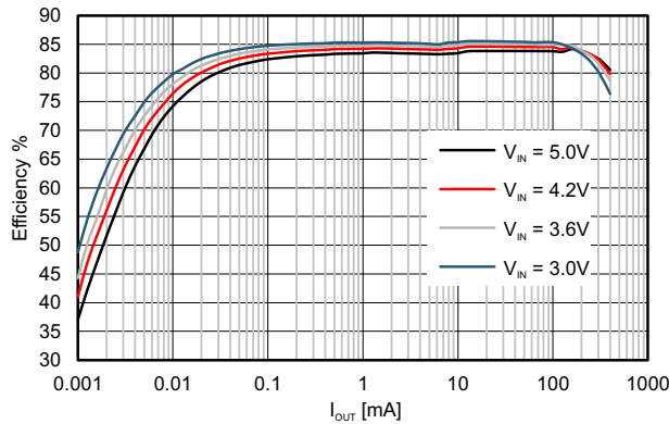
Figure 9-4. Efficiency vs Load Current; V_{OUT} = 1.2\text{ V}
