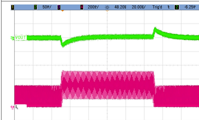
Figure 9-12. Load Transient Response; 100 mA to 290 mA
