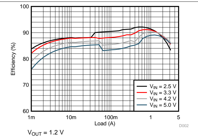
Figure 6. Efficiency
