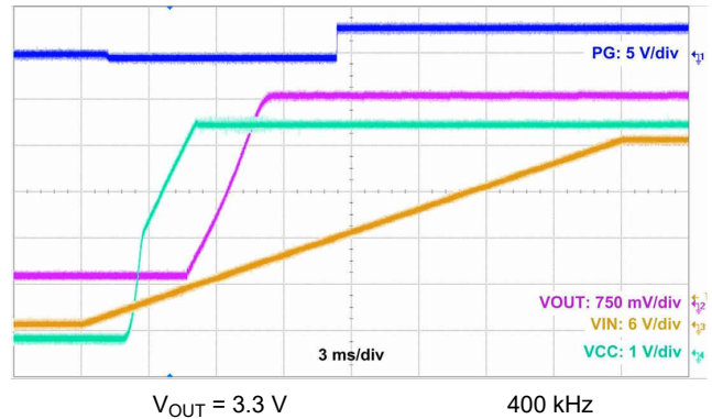
Figure 10-15. Start-Up Waveform
