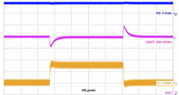
Figure 10-35. Load Transient
