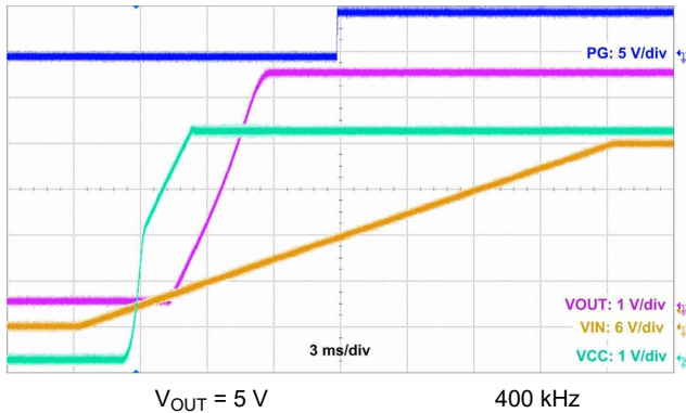
Figure 10-14. Start-Up Waveform
