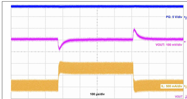
Figure 10-34. Load Transient
