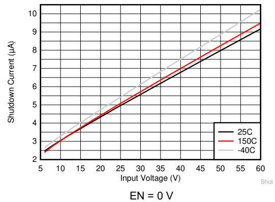
Figure 8-2. Shutdown Supply Current
