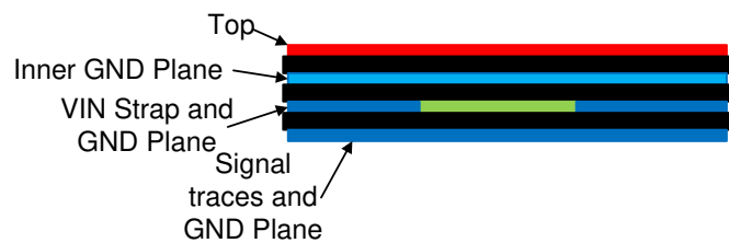
Figure 54. Example Layout
