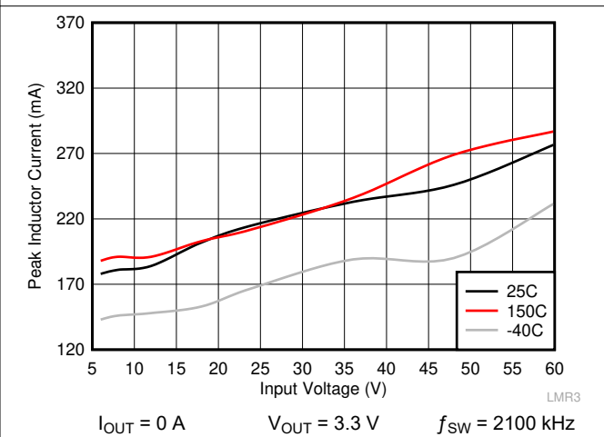
Figure 7-6. I PEAK-MIN
