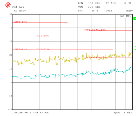
Figure 9-18. Conducted EMI vs. CISPR25 Limits (Yellow: Peak Signal, Blue: Average Signal)
