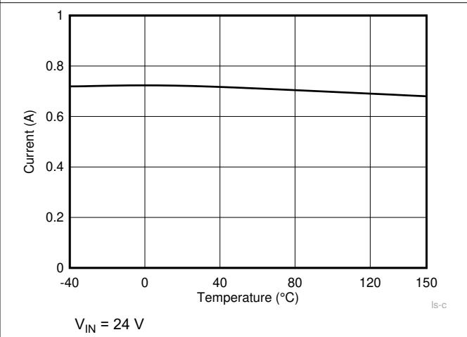
Figure 7-4. Low Side Current Limit
