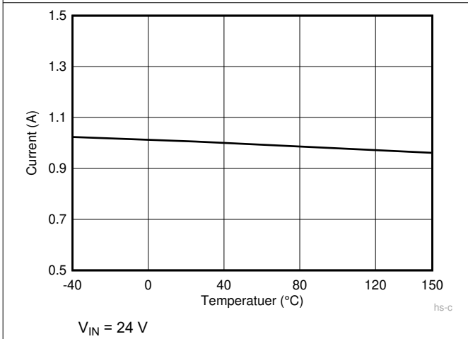
Figure 7-3. High Side Current Limit
