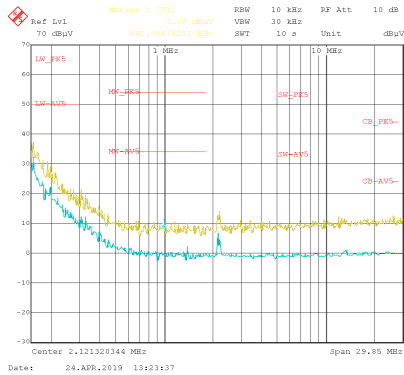
Figure 9-17. Conducted EMI vs. CISPR25 Limits (Yellow: Peak Signal, Blue: Average Signal)
