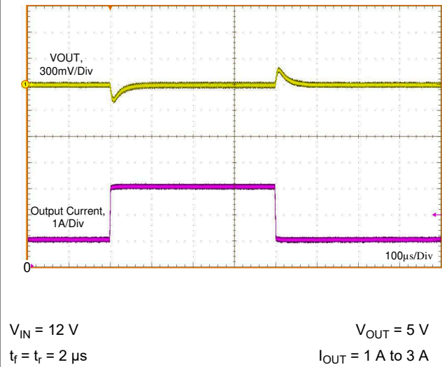
Figure 9-24. Load Transient
