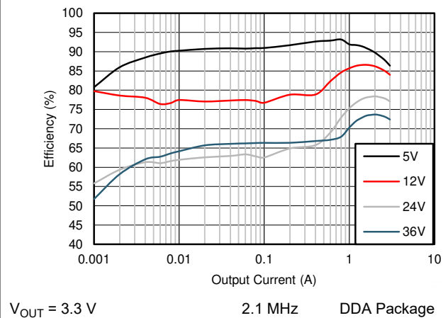
Figure 9-12. Efficiency
