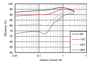
Efficiency versus Output Current V OUT = 5 V, 400 kHz, VQFN
