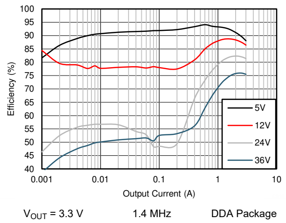
Figure 9-10. Efficiency
