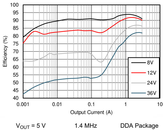
Figure 9-9. Efficiency
