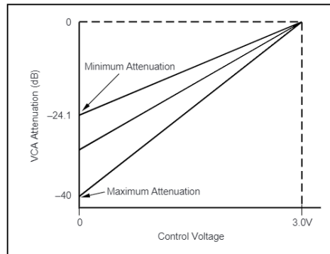
FIGURE 2. Swept Attenuator Characteristic.
