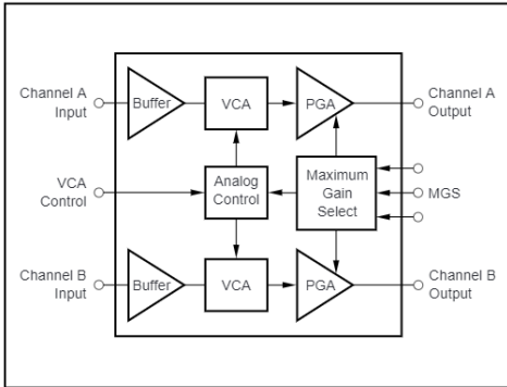
FIGURE 1. Simplified Block Diagram of the VCA2614.
