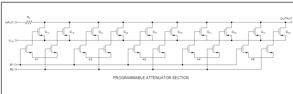
FIGURE 3. Programmable Attenuator Section.
