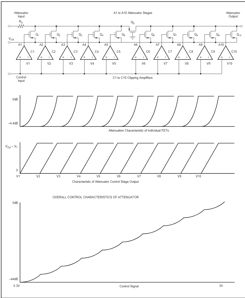
FIGURE 4. Piecewise Approximation to Logarithmic Control Characteristics.
