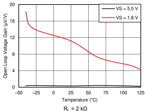
Figure 8-7. Open-Loop Gain vs Temperature
