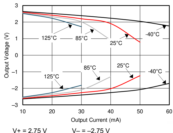
Figure 8-10. Output Voltage Swing vs Output Current
