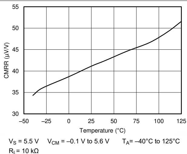
Figure 8-12. CMRR vs Temperature
