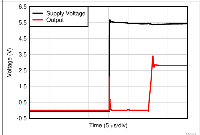
Figure 7-80. Turn-On Time
