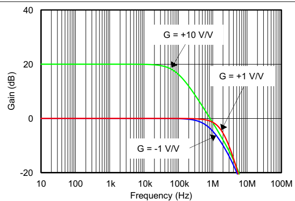
Figure 18. Closed-Loop Gain vs Frequency (Minimum Supply)
