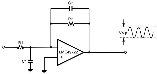
Figure 1. Wide Bandwidth Low Noise Low Drift Amplifier
