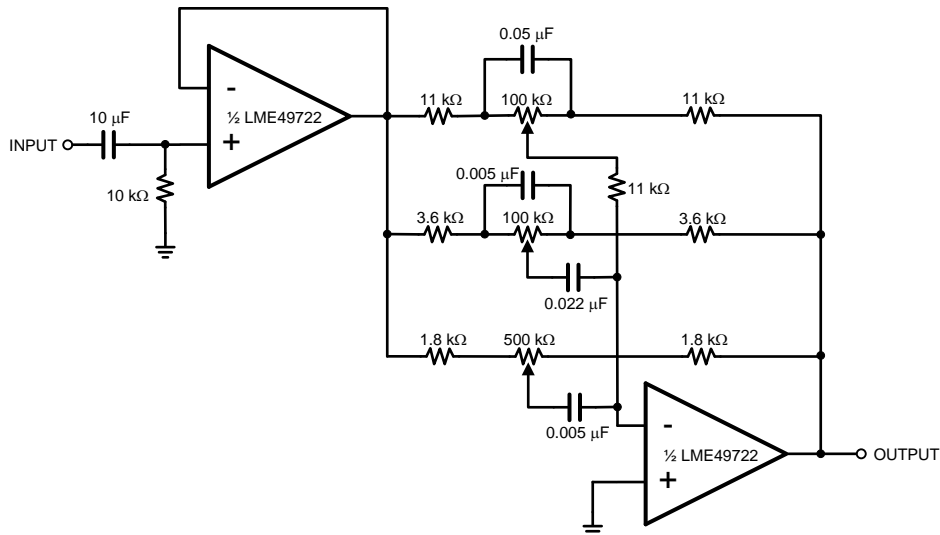
Figure 4. Three-Band Active Tone Control
