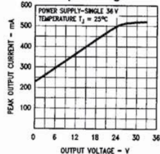
Peak Output Current vs Output Voltage
