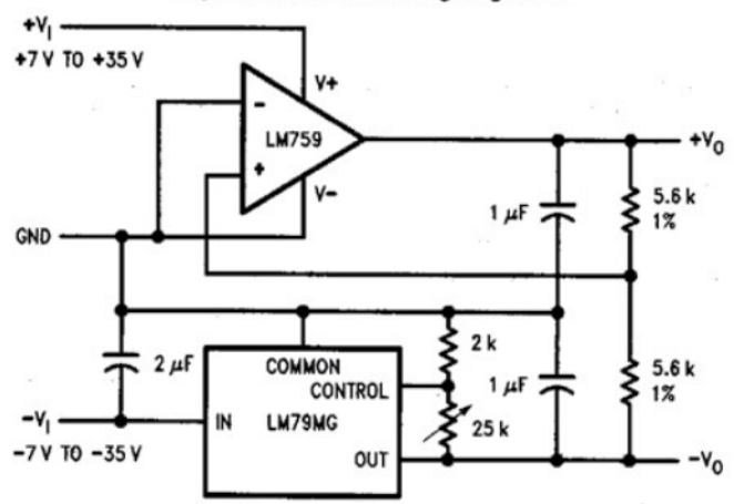
Adjustable Dual Tracking Regulator
