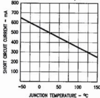
Short Circuit Current vs Junction Temperature
