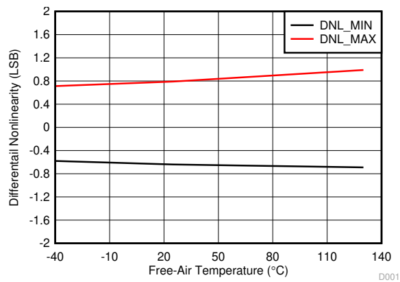
Figure 6-14. Typical DNL
