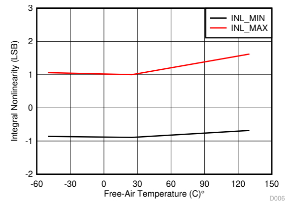
Figure 6-15. Typical INL
