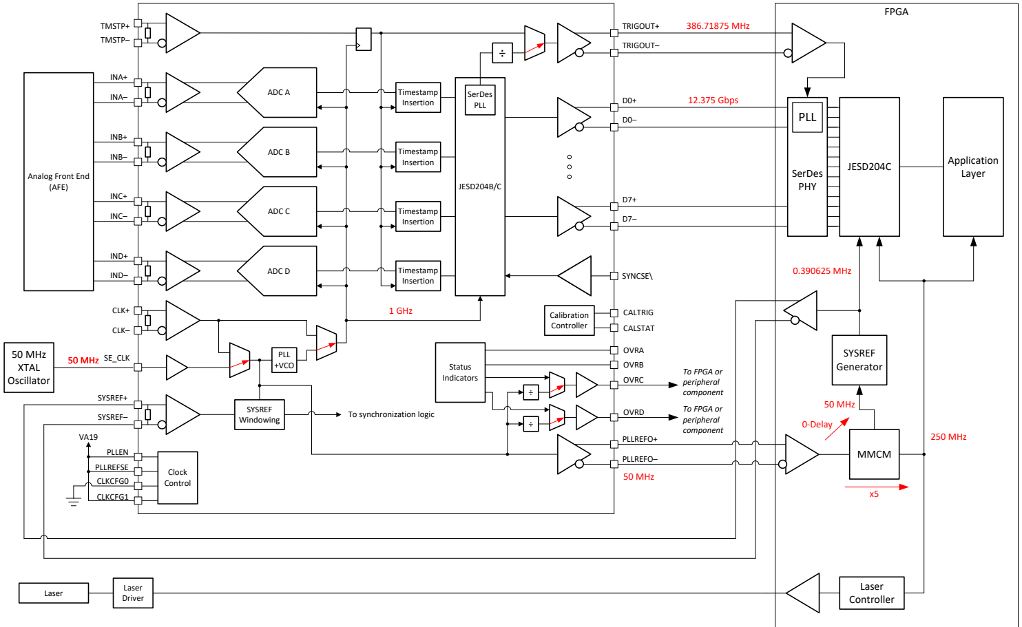
Figure 10-1. Typical Configuration for a LiDAR Digitizer
