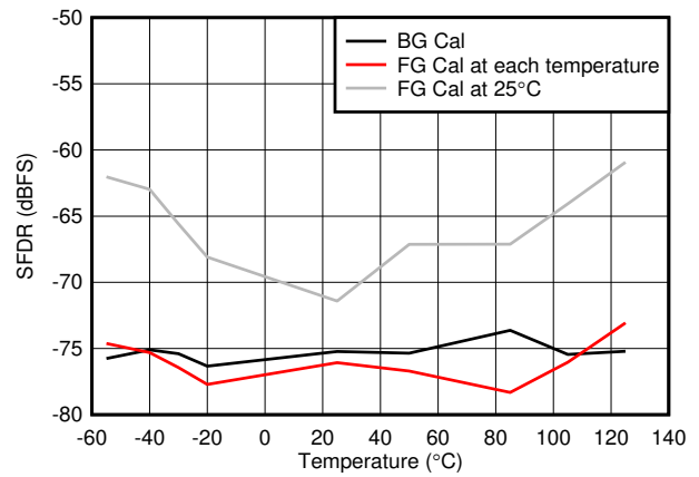
Worst spur is non-HD2 though -HD10 SDFR Figure 8-68. Worst Spur vs Temperature
