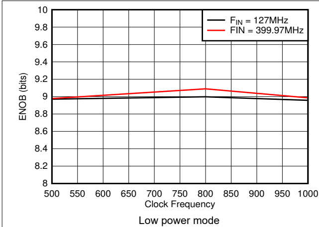
Figure 8-31. ENOB vs Sample Rate
