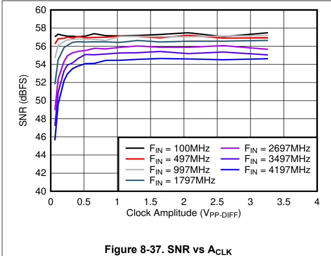
Figure 8-37. SNR vs A_{CLK}
