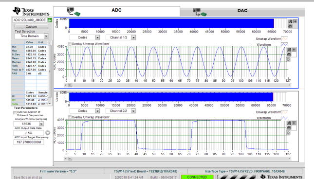
Figure 8-11. 200-MHz, Sine-Wave (Channel A) and 40-MHz, Square-Wave (Channel B) Time Domain for 5-GSPS, Single-Channel Oscilloscope
