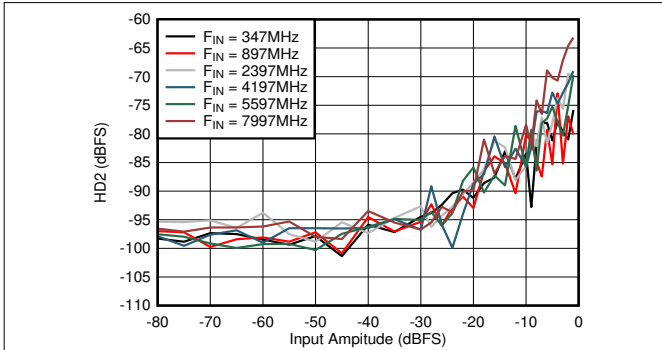
Figure 6-61. DES Mode: HD2 vs Input Amplitude and Frequency
