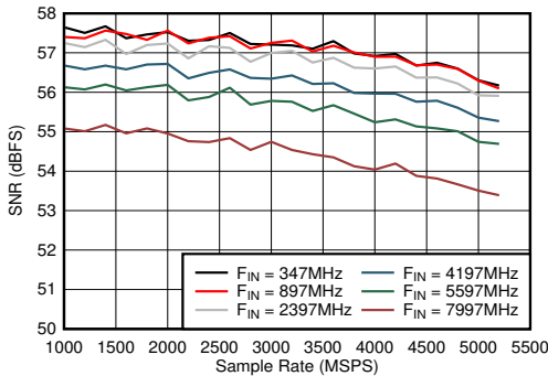
Figure 6-45. Dual Channel Mode: SNR vs Sample Rate and Input Frequency A_{IN} = -6\text{ dBFS}
