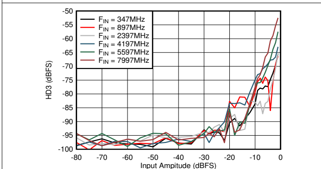
Figure 6-63. DES Mode: HD3 vs Input Amplitude and Frequency
