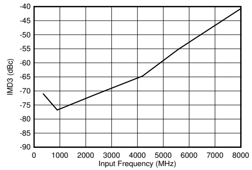
Figure 6-104. Dual Channel Mode: IMD3 vs Input Frequency
