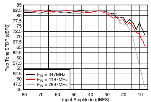
Figure 6-108. Dual Channel Mode: Two Tone SFDR vs Input Amplitude
