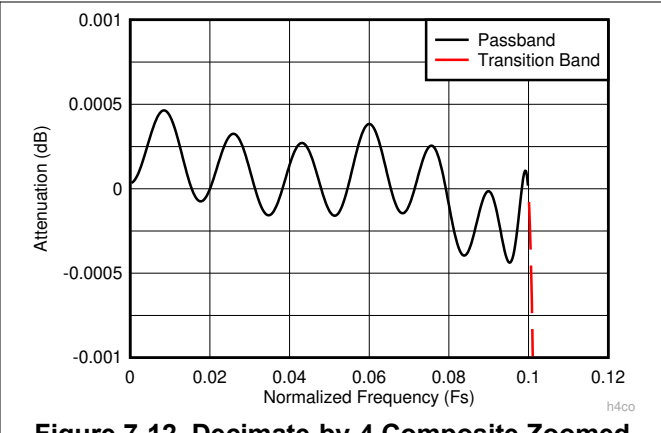
Figure 7-12. Decimate-by-4 Composite Zoomed Pass-Band Response h4co
