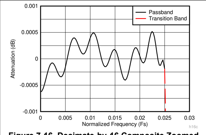
Figure 7-16. Decimate-by-16 Composite Zoomed Pass-Band Response h16c
