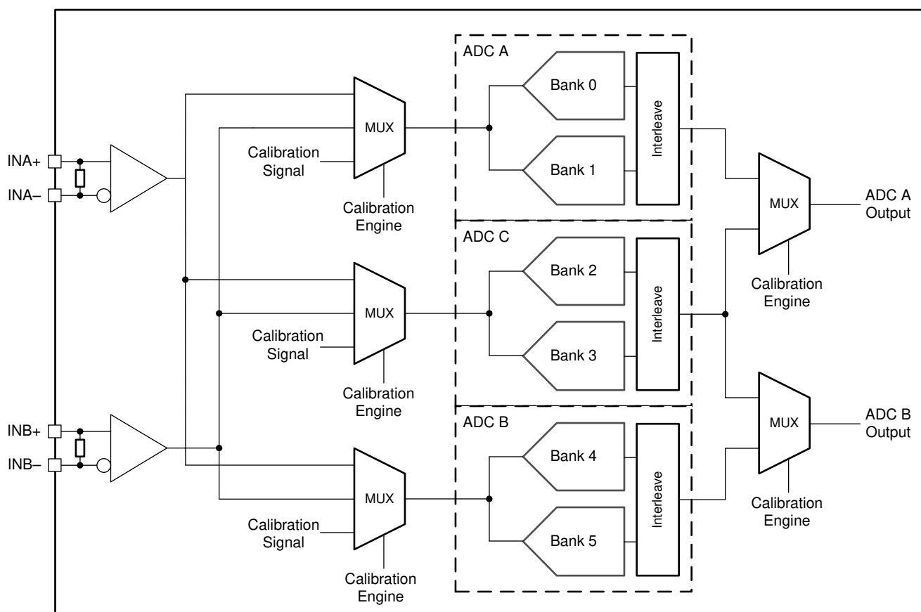
Figure 7-25. ADC12DJ5200RF Calibration System Block Diagram
