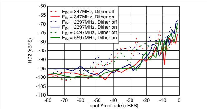
Figure 6-62. DES Mode: HD2 vs Input Amplitude and Dither
