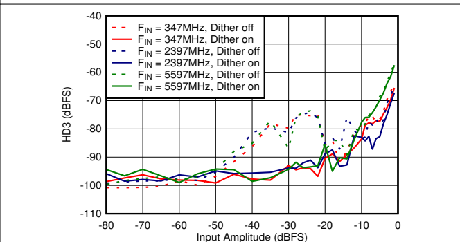
Figure 6-64. DES Mode: HD3 vs Input Amplitude and Dither
