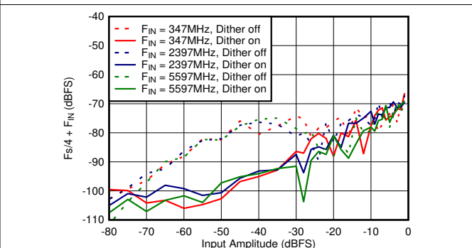
Figure 6-66. DES Mode: F_s/4 - F_{\text{IN}} vs Input Amplitude and Dither
