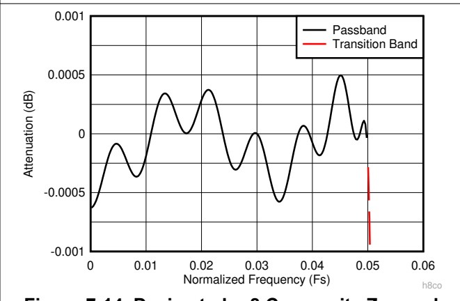
Figure 7-14. Decimate-by-8 Composite Zoomed Pass-Band Response h8co
