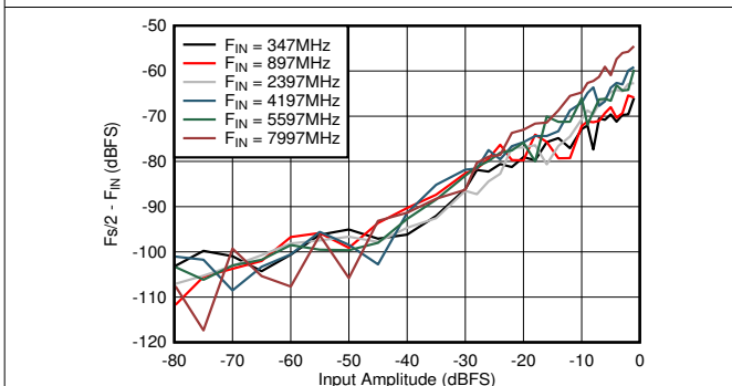
Figure 6-65. DES Mode: F_s/2 - F_{\text{IN}} vs Input Amplitude and Frequency
