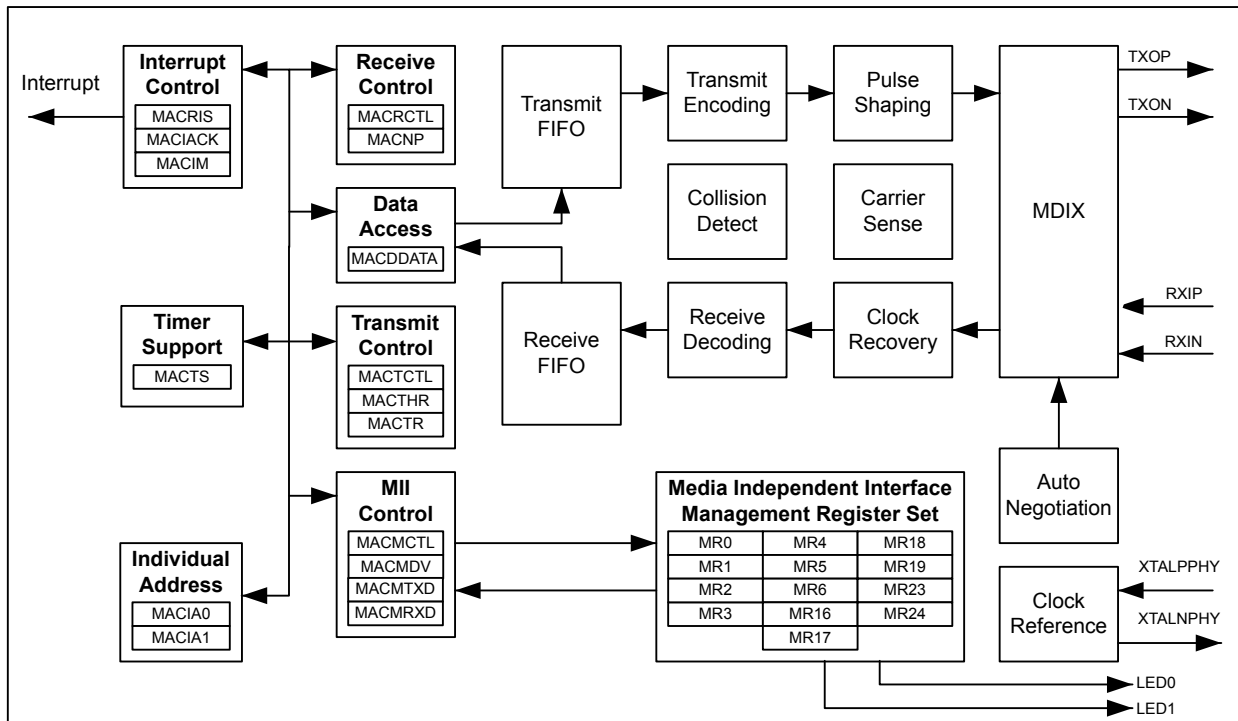
Figure 16-2. Ethernet Controller Block Diagram
