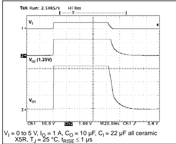
Figure 31. Start-up transient
