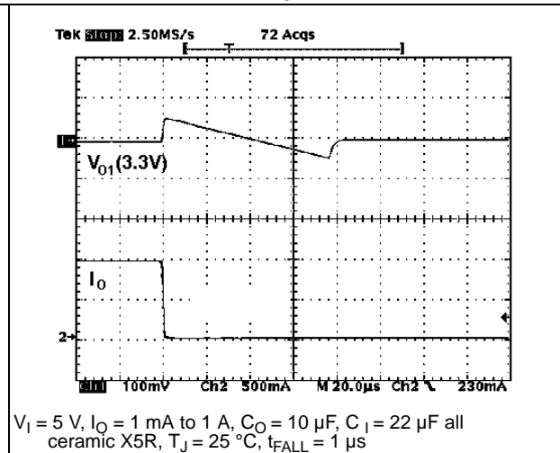
Figure 30. Change of V_O with step load change
