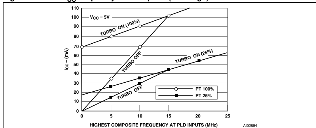
Figure 70. PLD I_{CC} /frequency consumption (5 V range)
