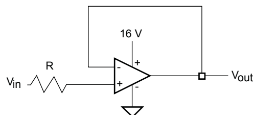
Figure 36. Input current limitation
