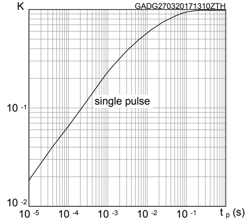
Figure 2. Thermal impedance
