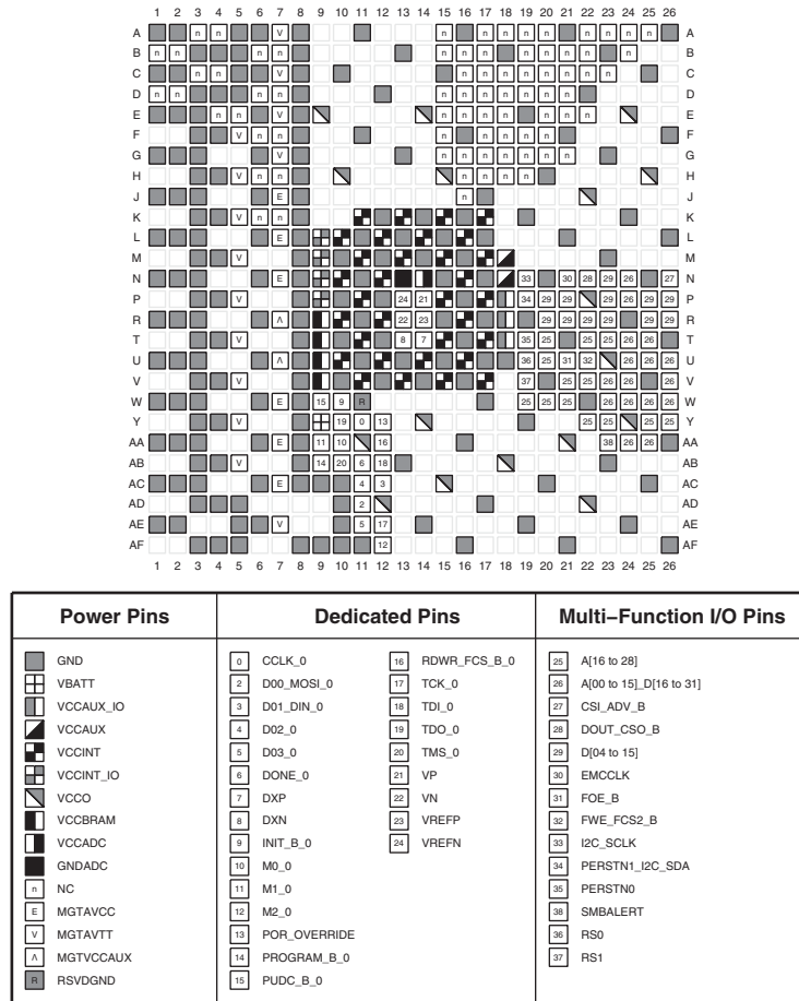
Figure 3-78: FFVB676 Package— XCAU10P Configuration/Power Diagram
