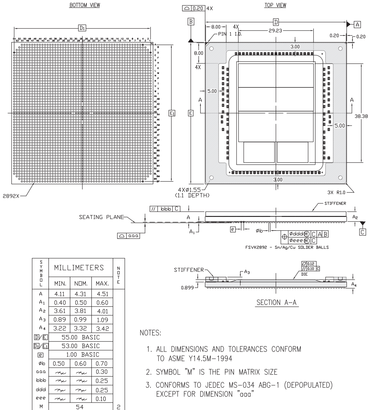
Figure 4-64: Package Dimensions for FSVK2892 (XCVU57P)
