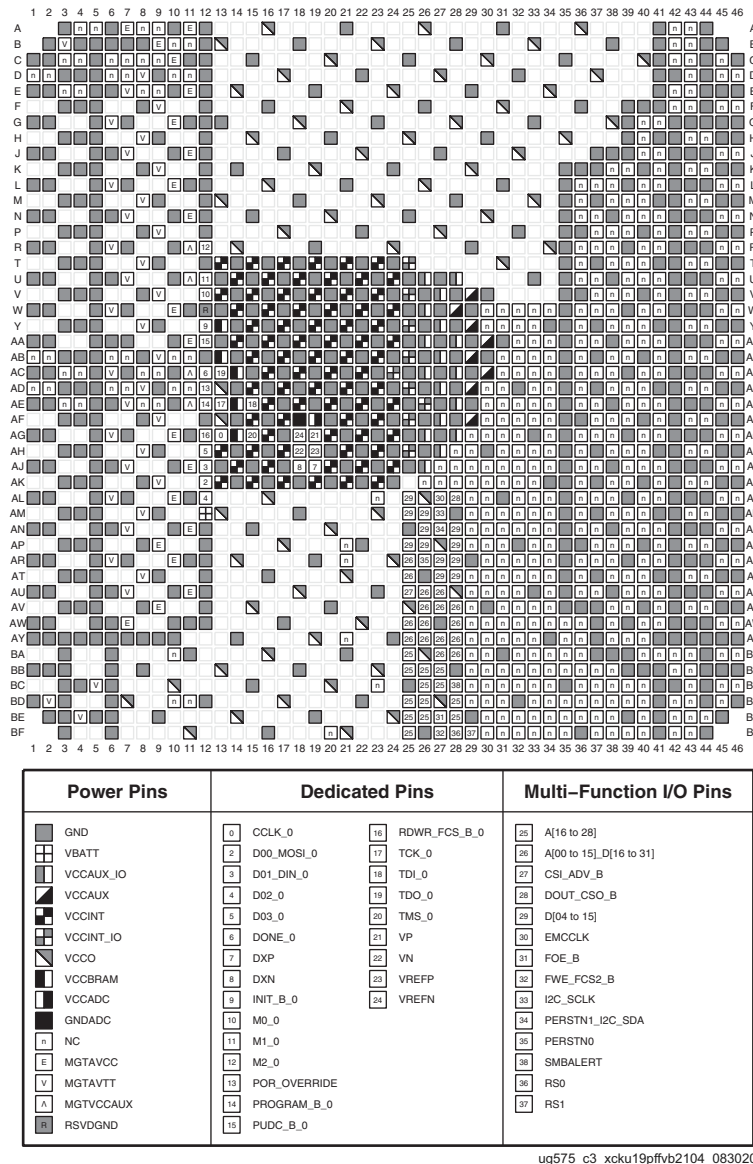
Figure 3-125: FFVB2104 Package—XCKU19P Configuration/Power Diagram
