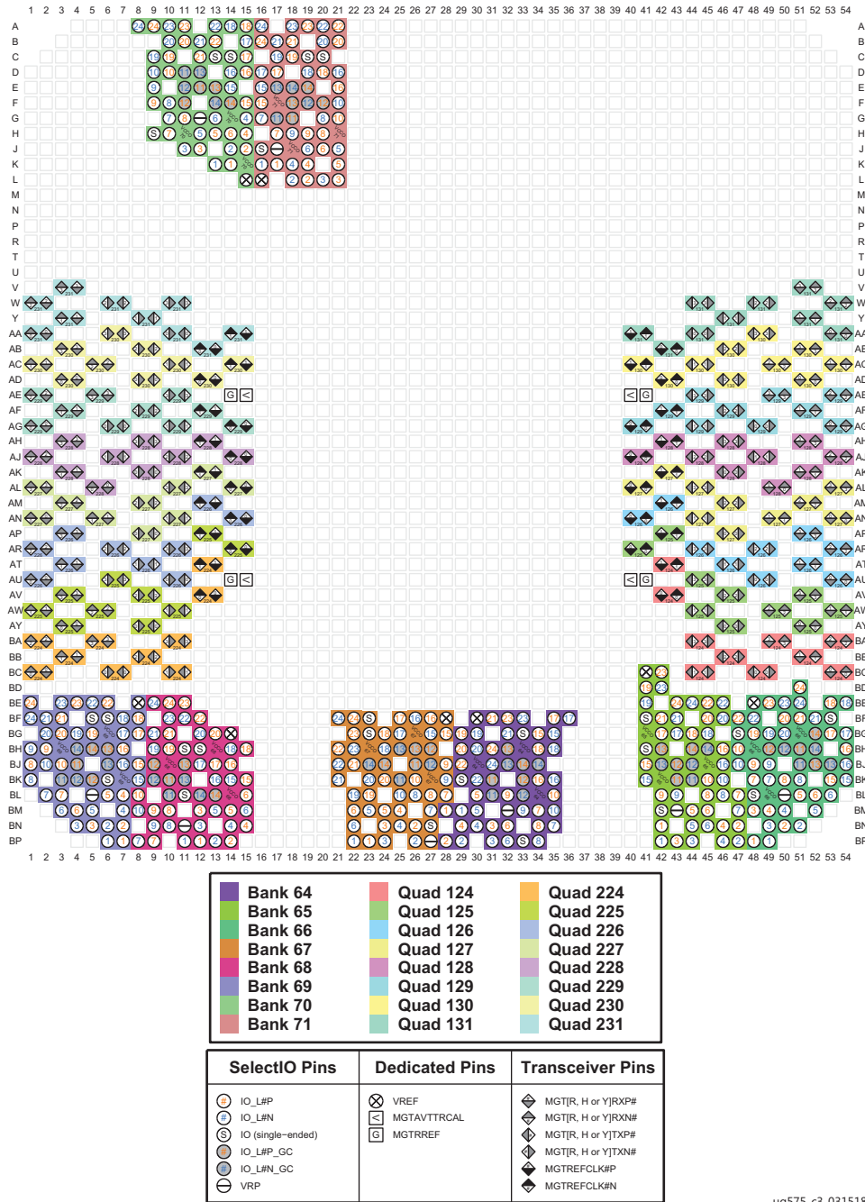
Figure 3-181: FSVH2892 Package—XCVU35P and XCVU45P I/O Bank Diagram
