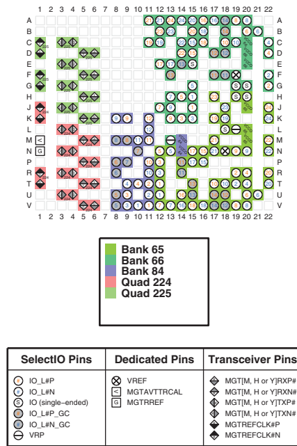
Figure 3-95: UBVA368 Package—XCAU15P I/O Bank Diagram
