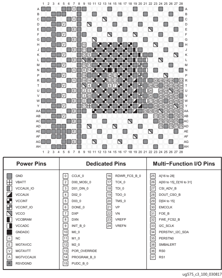
Figure 3-102: SFVB784 Package—XCKU3P and XCKU5P and SFRB784 Package—XQKU5P Configuration/Power Diagram
