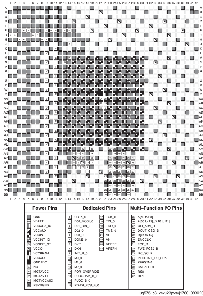
Figure 3-130: FSVJ1760 Package—XCVU23P Configuration/Power Diagram
