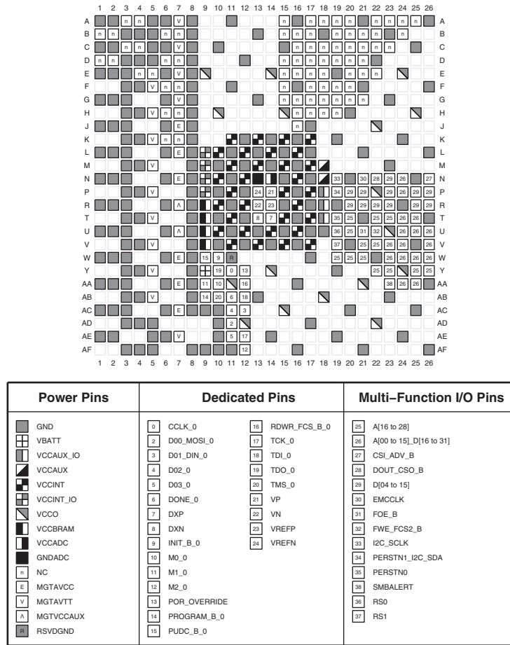
Figure 3-80: FFVB676 Package— XCAU15P Configuration/Power Diagram
