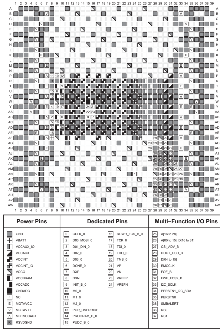
Figure 3-128: FVC1517 Package—XCVU3P and FRC1517 Package—XQVU3P Configuration/Power Diagram
