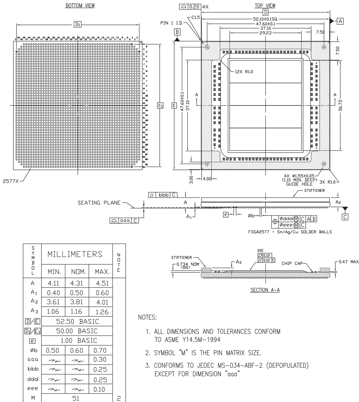
Figure 4-60: Package Dimensions for FSGA2577 (XCVU13P, XCVU27P, and XCVU29P)
