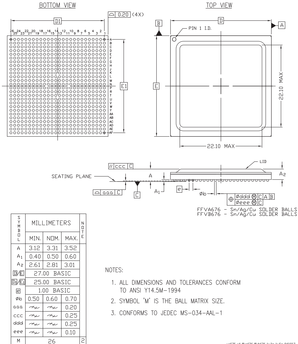
Figure 4-5: Package Dimensions for FFVA676 (XCKU3P and XCKU5P) and FFVB676 (XCAU10P, XCAU15P, XCAU20P, and XCAU25P)
