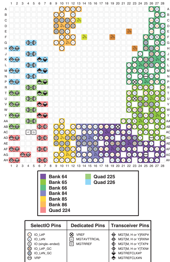
Figure 3-89: SFVB784 Package—XCAU20P I/O Bank Diagram
