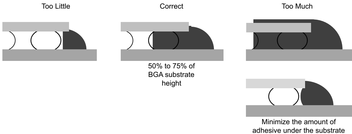
Figure 9-2: Edge Bonding Adhesive Placement Parameters
