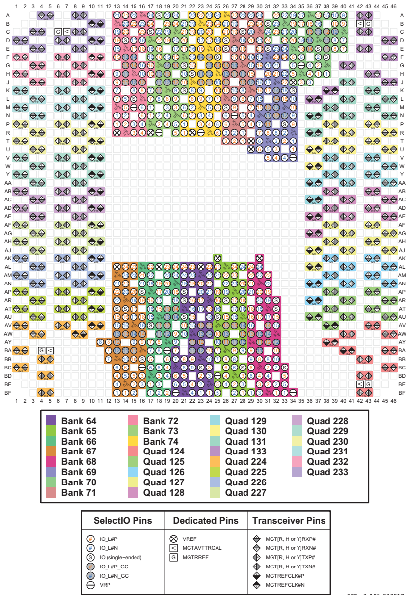
Figure 3-145: FLGB2104 Package—XCVU11P I/O Bank Diagram
