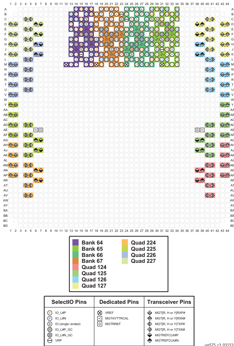
Figure 3-133: FSVH1924 Package—XCVU31P I/O Bank Diagram
