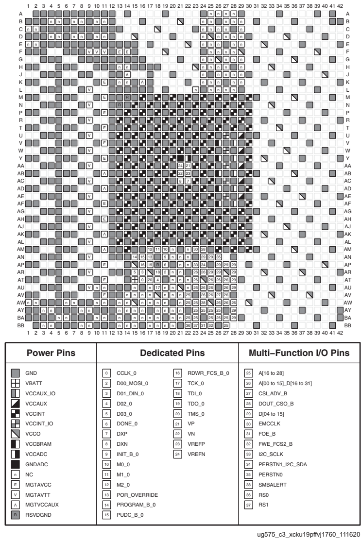
Figure 3-123: FFVJ1760 Package—XCKU19P Configuration/Power Diagram
