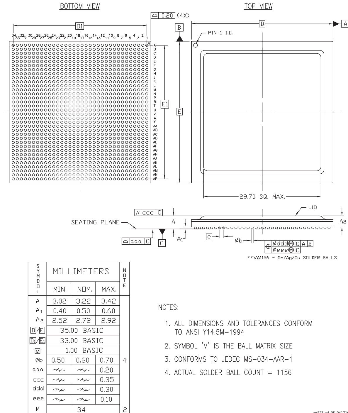
Figure 4-14: Package Dimensions for FFVA1156 (XCKU025, XCKU035, and XCKU040)
