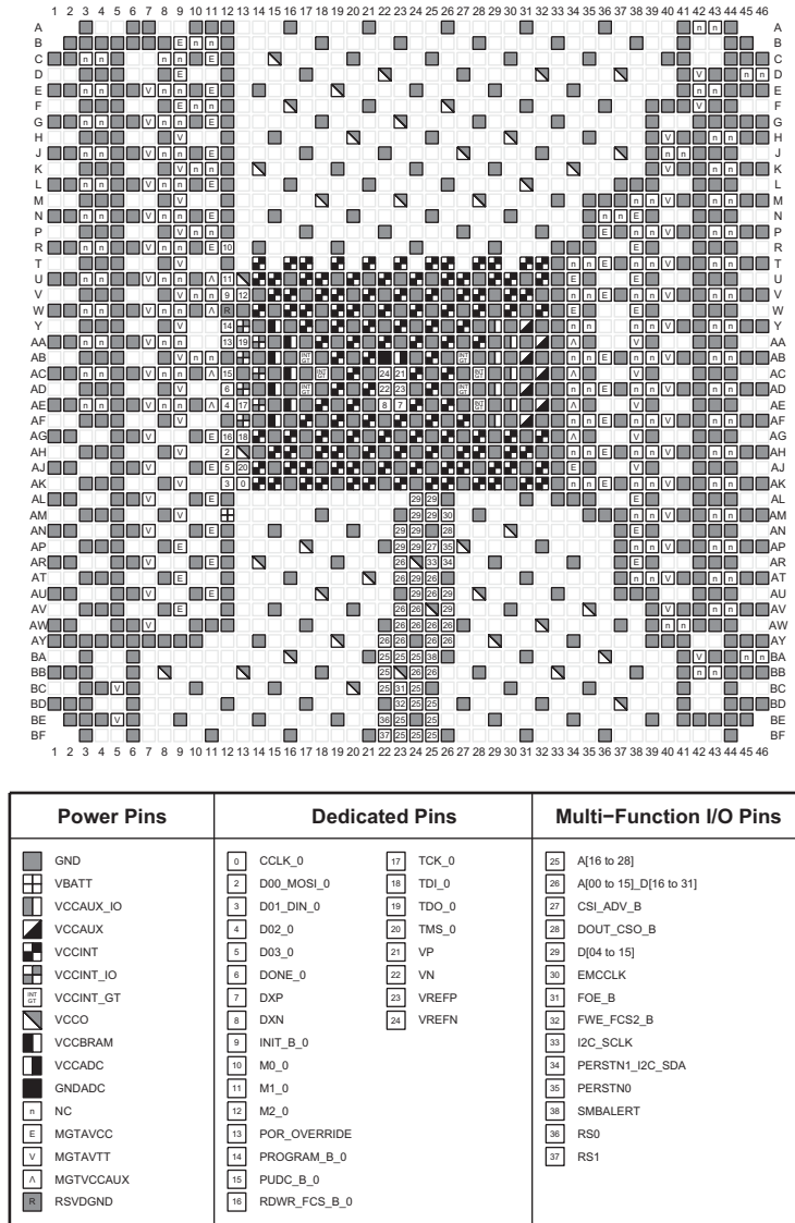
Figure 3-164: FIGD2104 Package—XC7VU27P Configuration/Power Diagram
