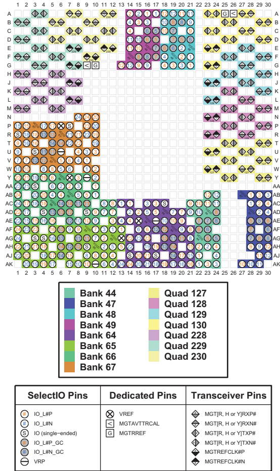
Figure 3-109: FFVE900 Package—XCKU13P I/O Bank Diagram
