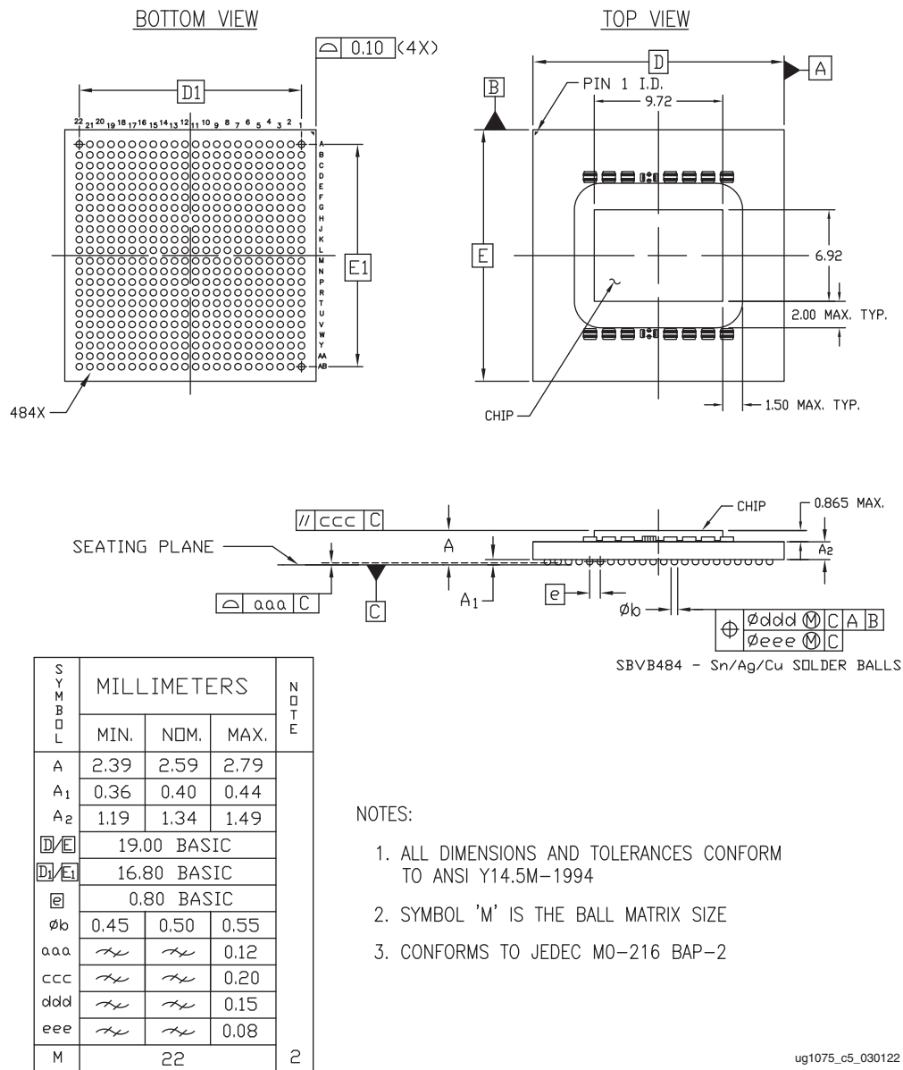
Figure 4-2: Package Dimensions for SBVB484 (XCAU10P and XCAU15P)
