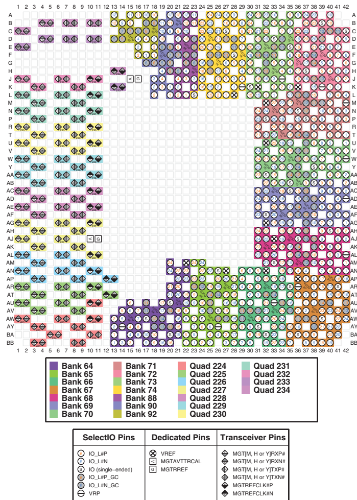
Figure 3-129: FSVJ1760 Package—XCVU23P I/O Bank Diagram
