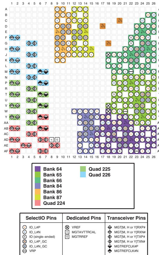
Figure 3-81: FFVB676 Package—XCAU20P I/O Bank Diagram
