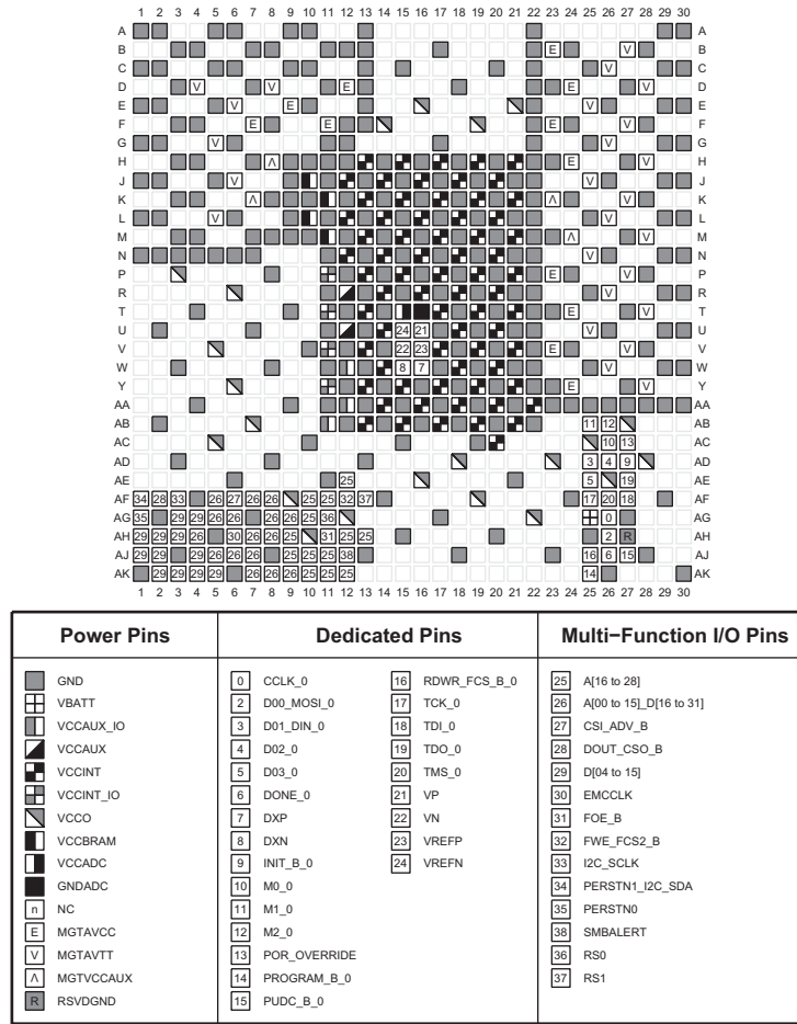
Figure 3-110: FFVE900 Package—XCKU13P Configuration/Power Diagram
