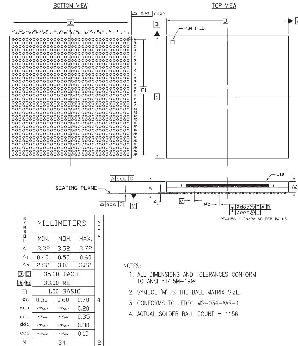
Figure 4-19: Package Dimensions for RFA1156 (XQKU060 and XQKU095)
