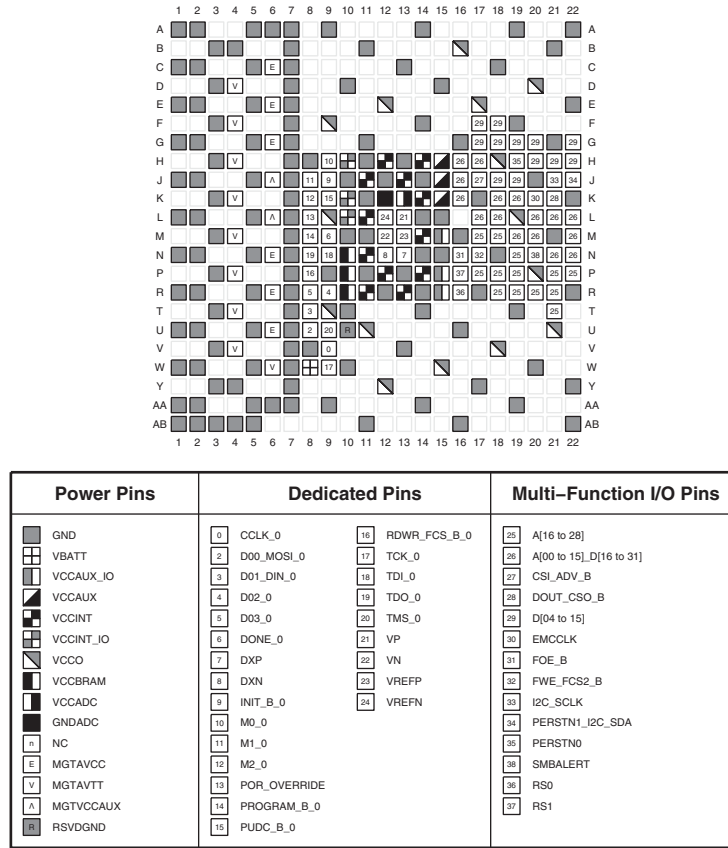
Figure 3-88: SBVB484 Package— XCAU15P Configuration/Power Diagram
