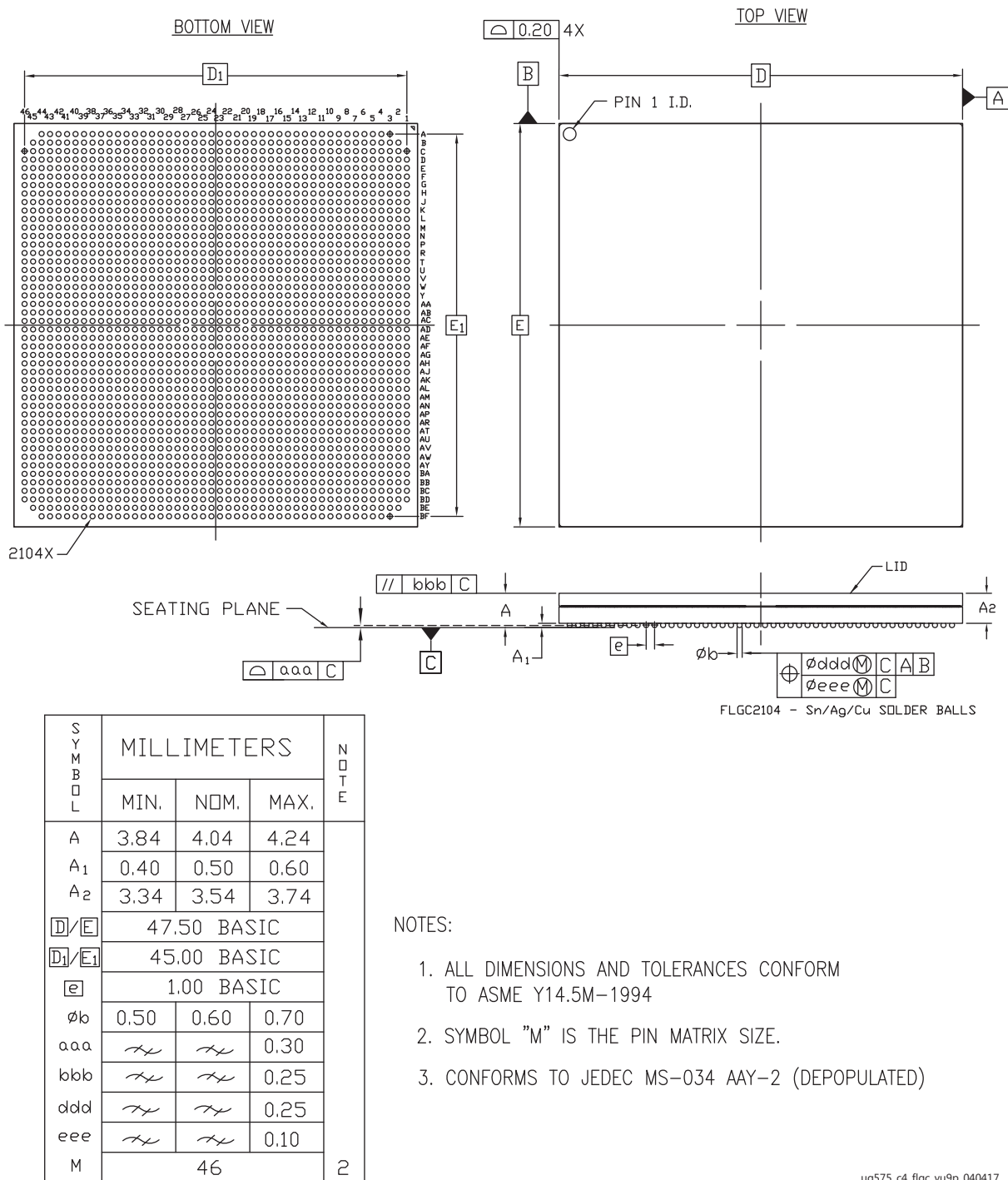
Figure 4-48: Package Dimensions for FLGC2104 (XCVU9P)
