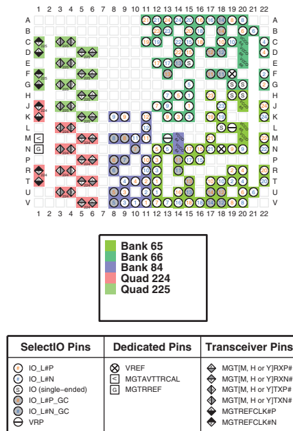
Figure 3-93: UBVA368 Package—XCAU10P I/O Bank Diagram
