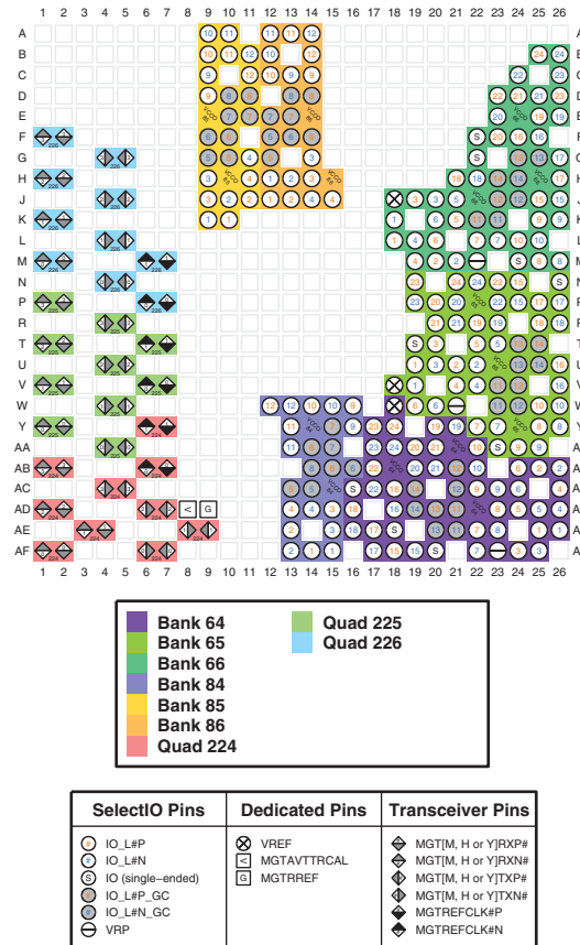
Figure 3-79: FFVB676 Package—XCAU15P I/O Bank Diagram
