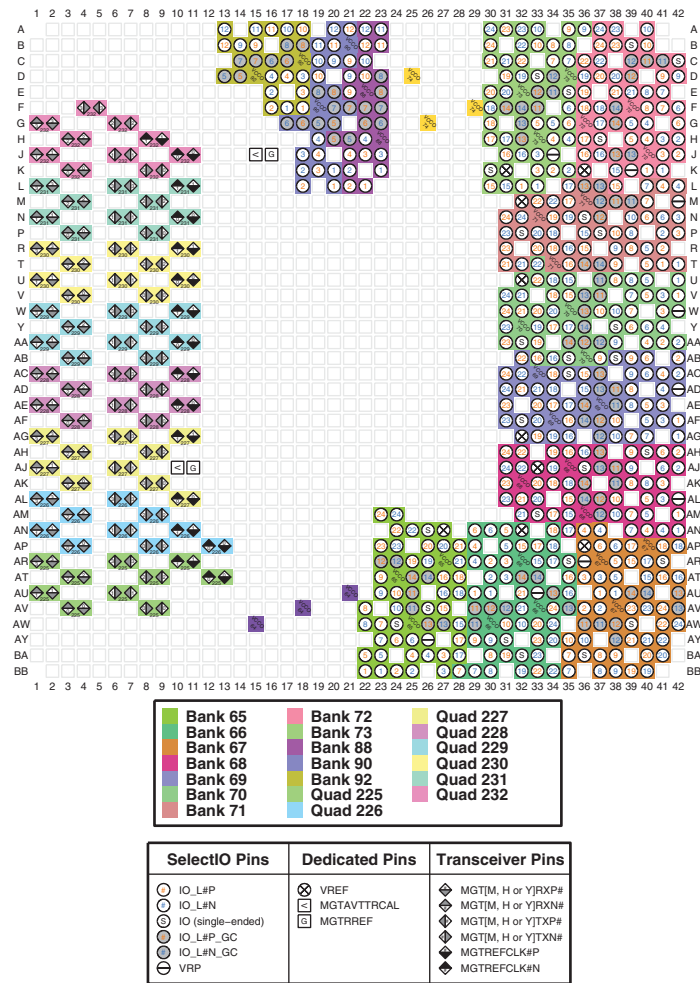
Figure 3-122: FFVJ1760 Package—XCKU19P I/O Bank Diagram
