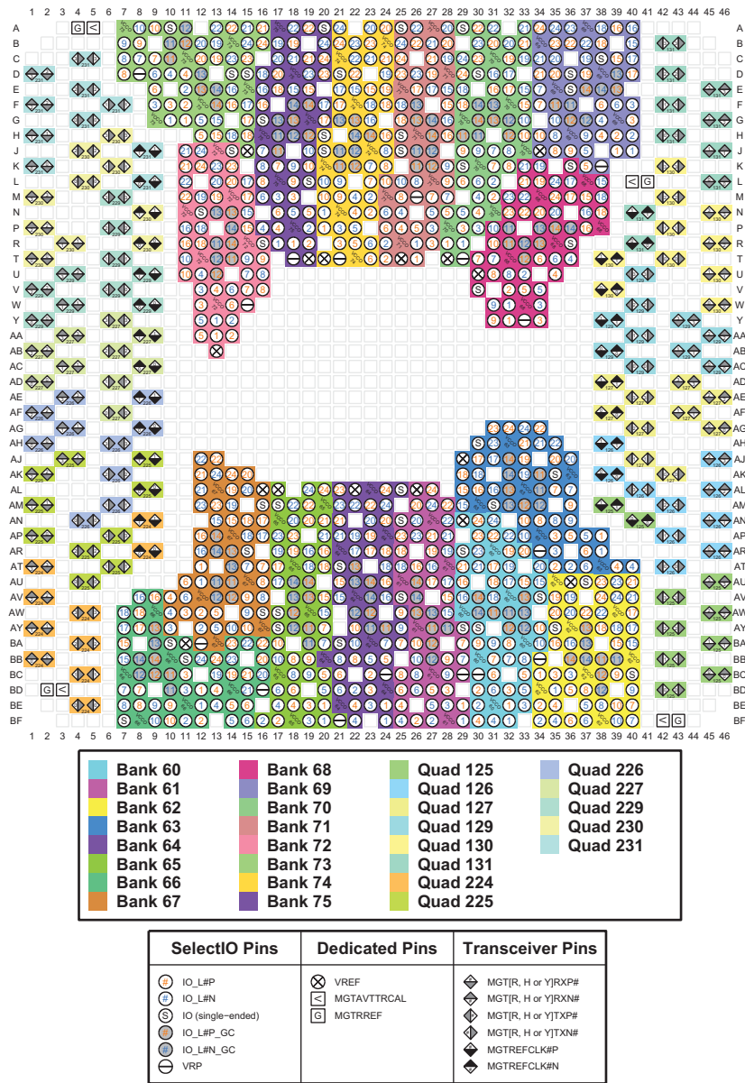
Figure 3-139: FHGA2104 Package—XCVU13P I/O Bank Diagram
