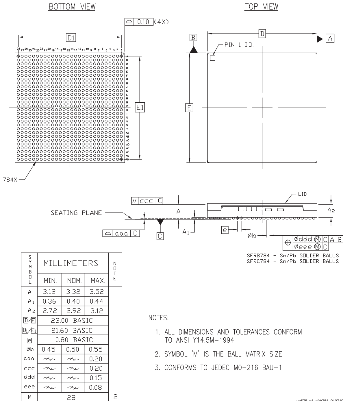
Figure 4-10: Package Dimensions for SFRB784 (XQKU5P)
