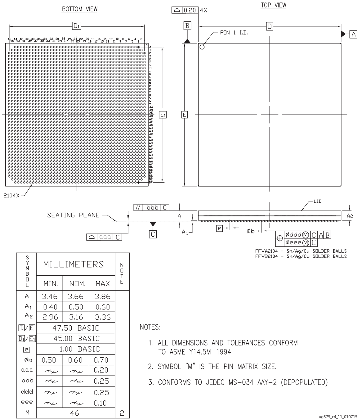
Figure 4-36: Package Dimensions for FFVA2104 (XCVU080, and XCVU095) and FFVB2104 (XCKU095, XCVU080, and XCVU095)
