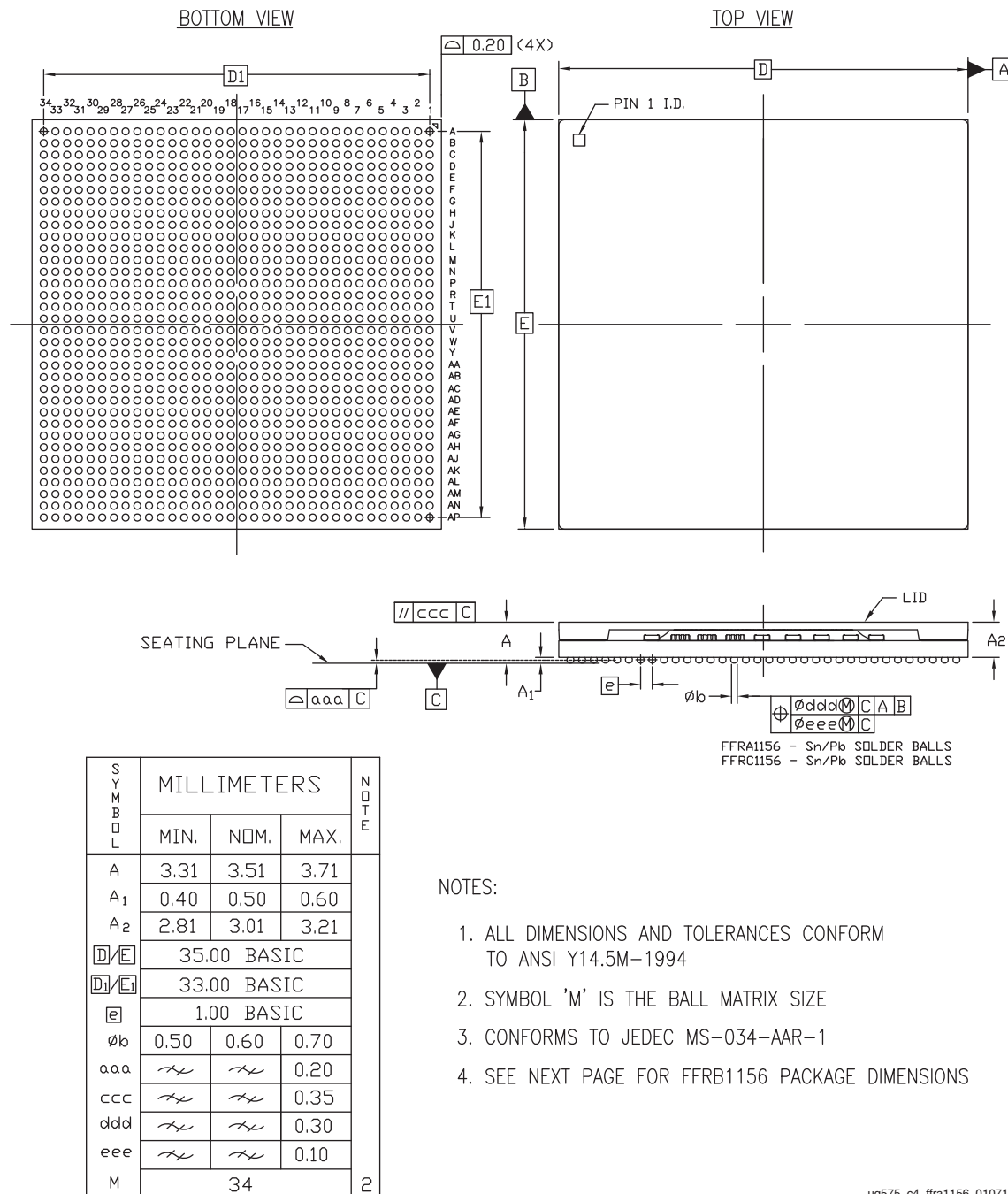
Figure 4-17: Package Dimensions for FFRA1156 (XQKU15P)
