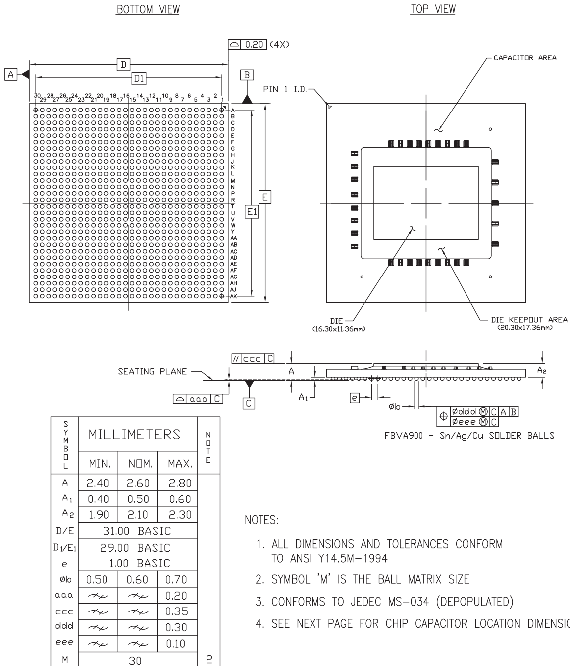
Figure 4-11: Package Dimensions for FBVA900 (XCKU035 and XCKU040)
