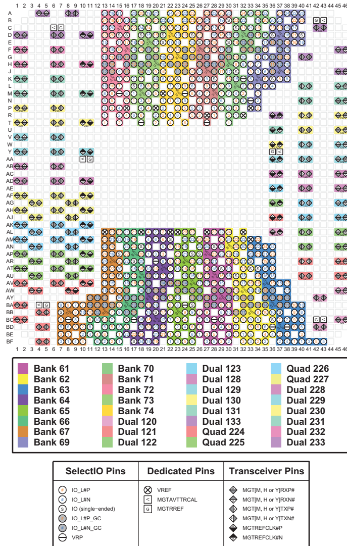
Figure 3-163: FIGD2104 Package—XCVU27P I/O Bank Diagram
