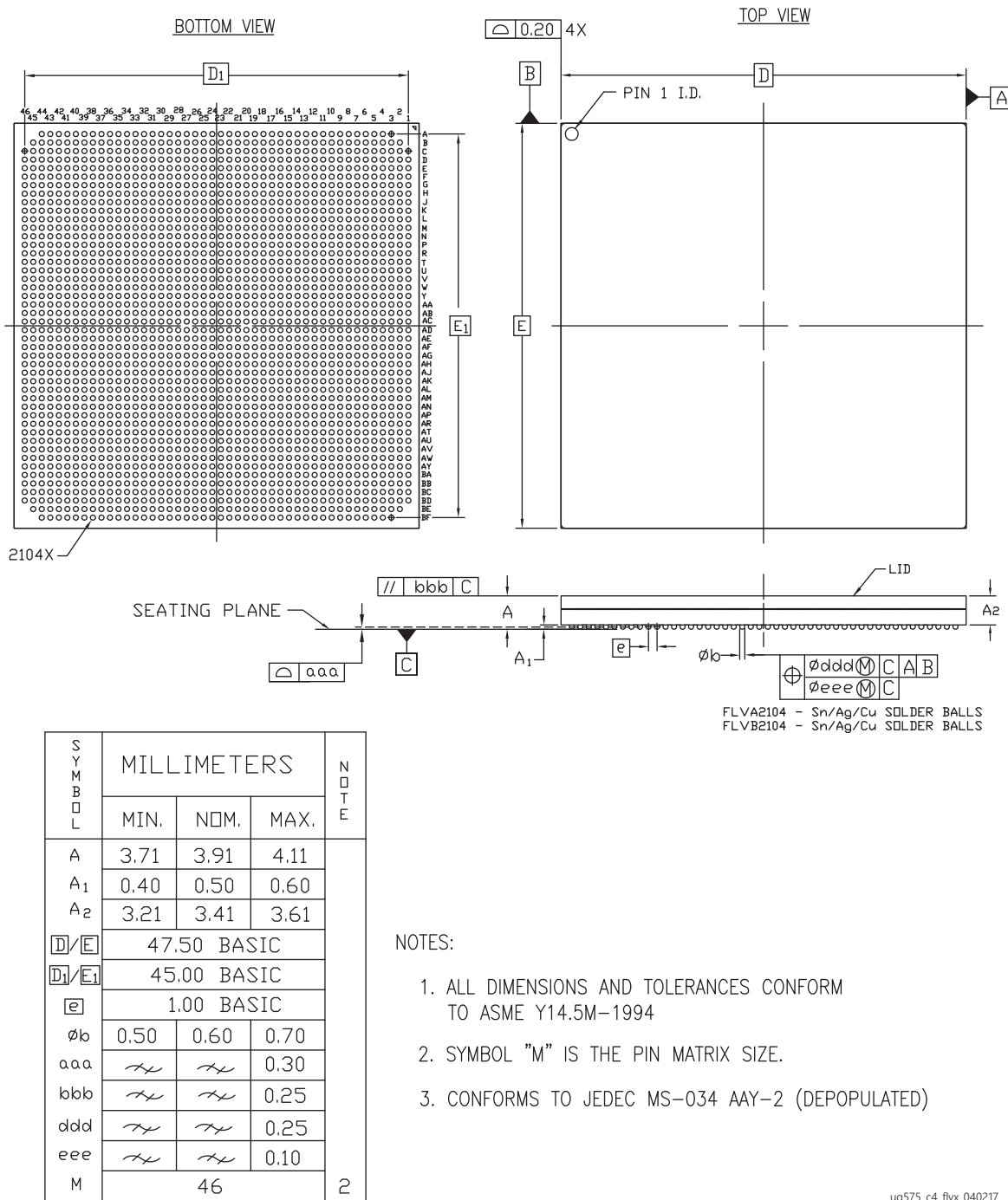
Figure 4-41: Package Dimensions for FLVA2104 (XCVU5P and XCVU7P) and FLVB2104 (XCVU5P and XCVU7P)
