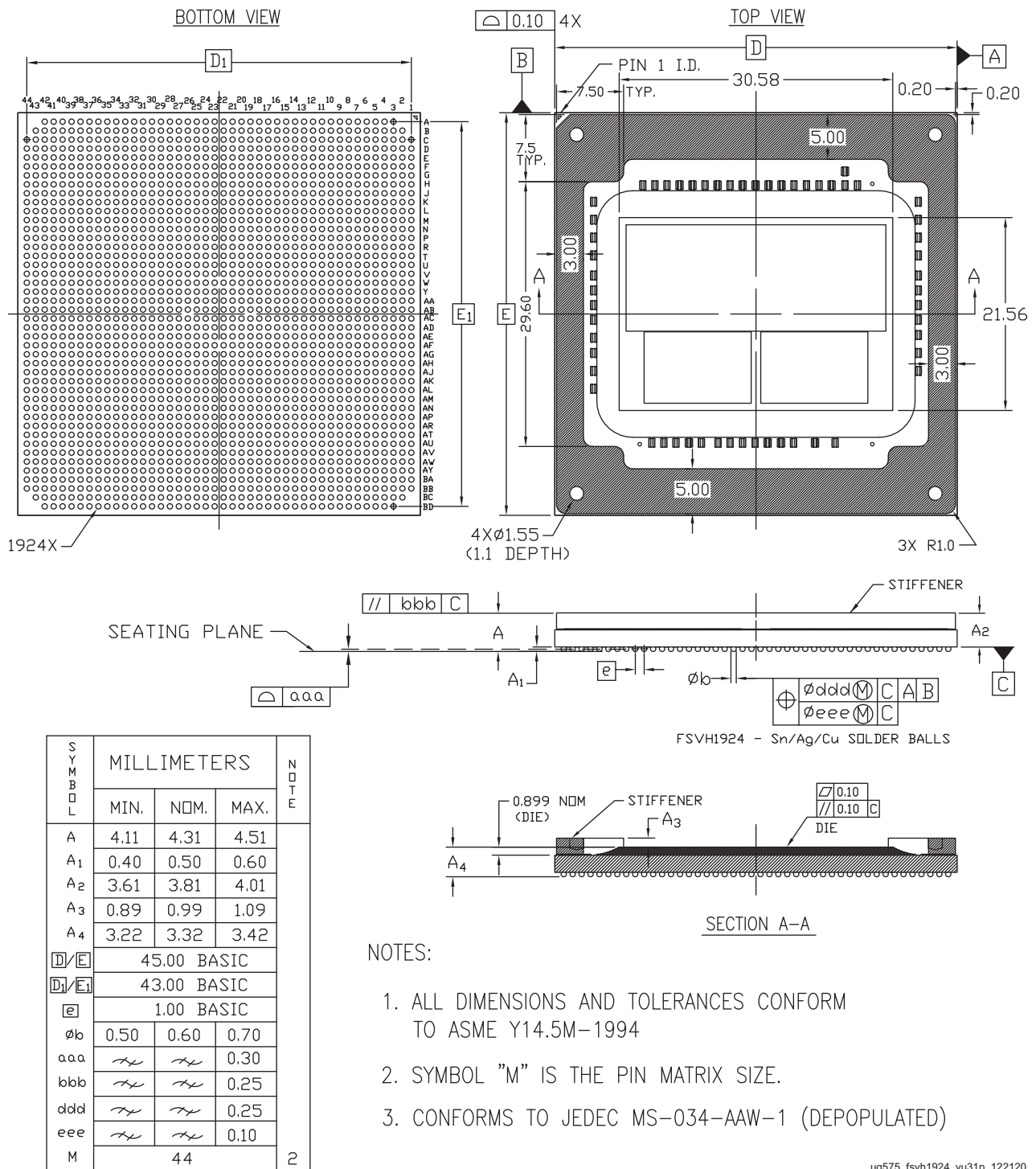
Figure 4-35: Package Dimensions for FSVH1924 (XCVU31P)
