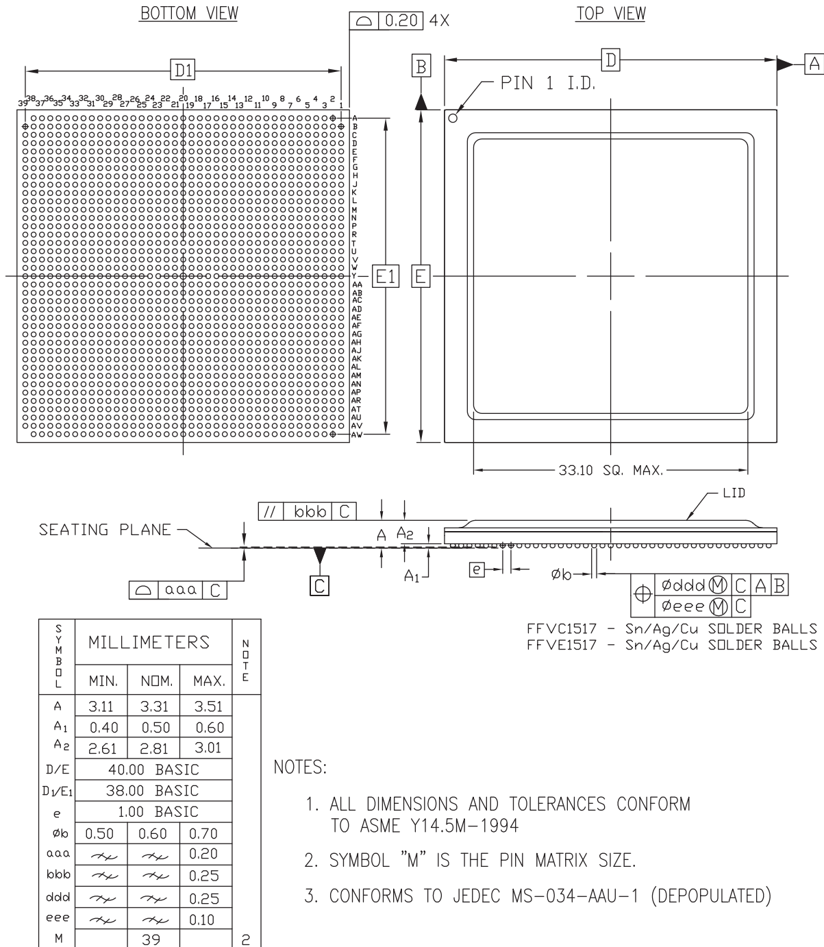
Figure 4-22: Package Dimensions for FFVC1517 (XCVU3P) and FFVE1517 (XCKU11P and XCKU15P)
