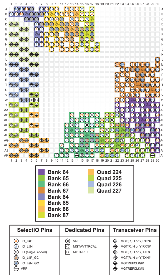
Figure 3-103: FFVD900 Package—XCKU3P and XCKU5P I/O Bank Diagram
