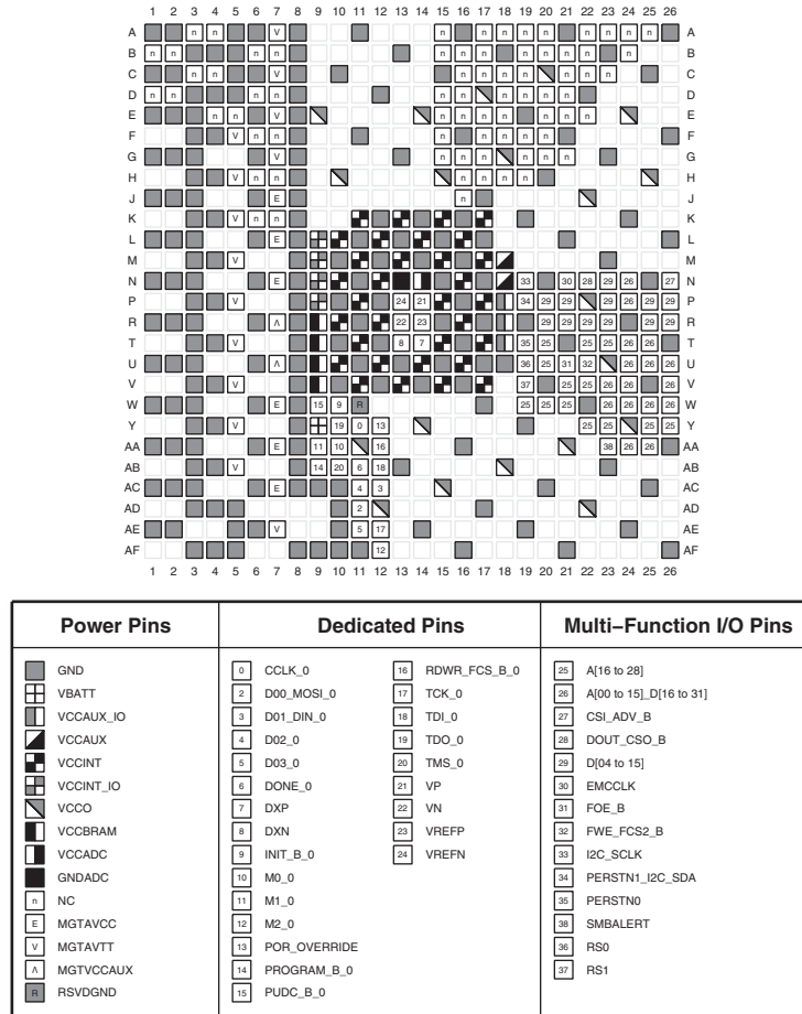
Figure 3-82: FFVB676 Package— XCAU20P Configuration/Power Diagram
