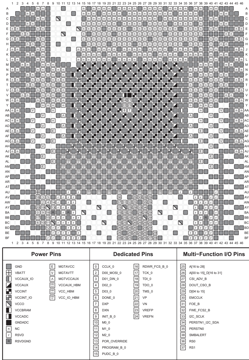
Figure 3-168: FSVH2104 Package—XCVU33P Configuration/Power Diagram
