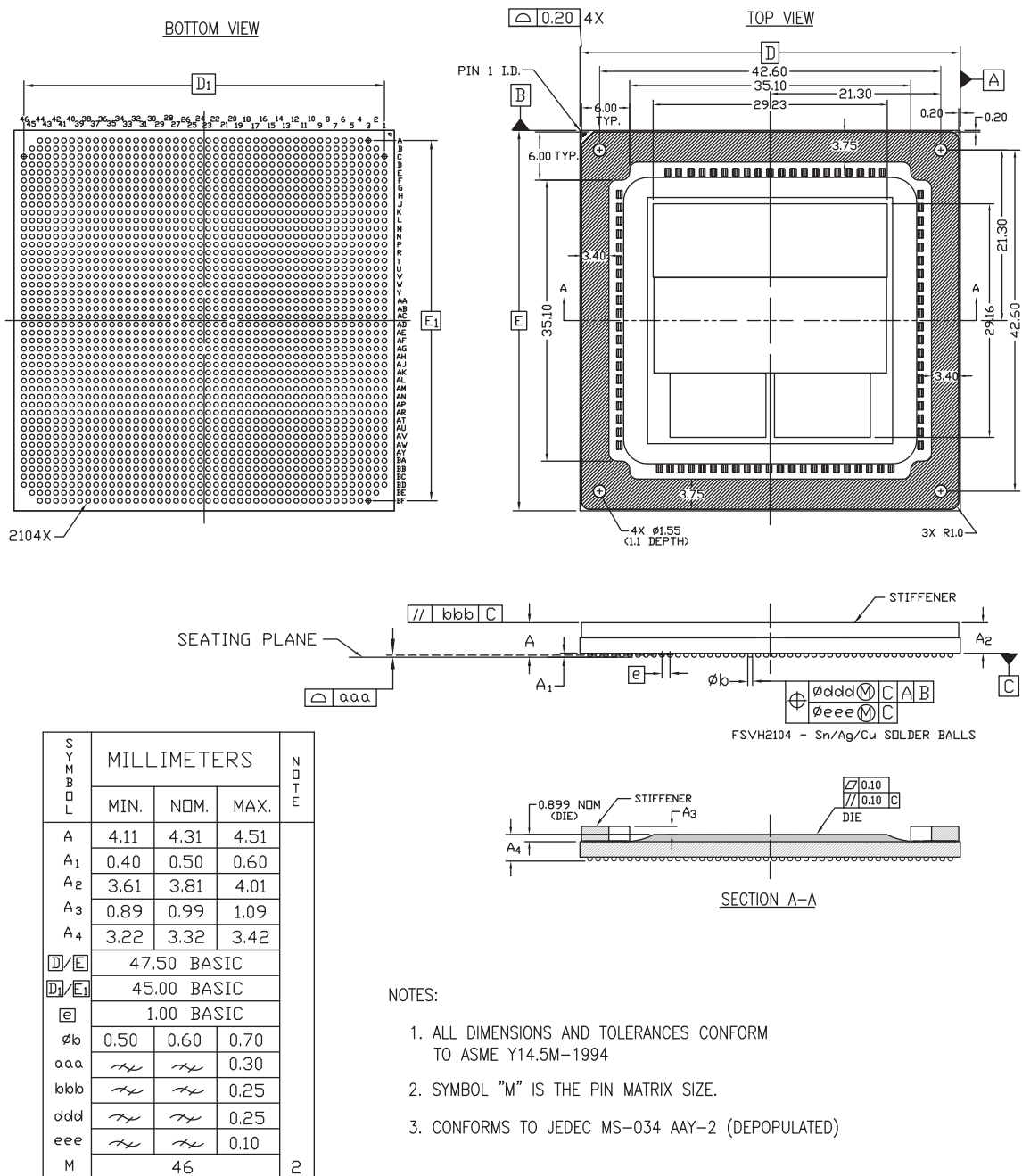
Figure 4-55: Package Dimensions for FSVH2104 (XCVU35P and XCVU45P)
