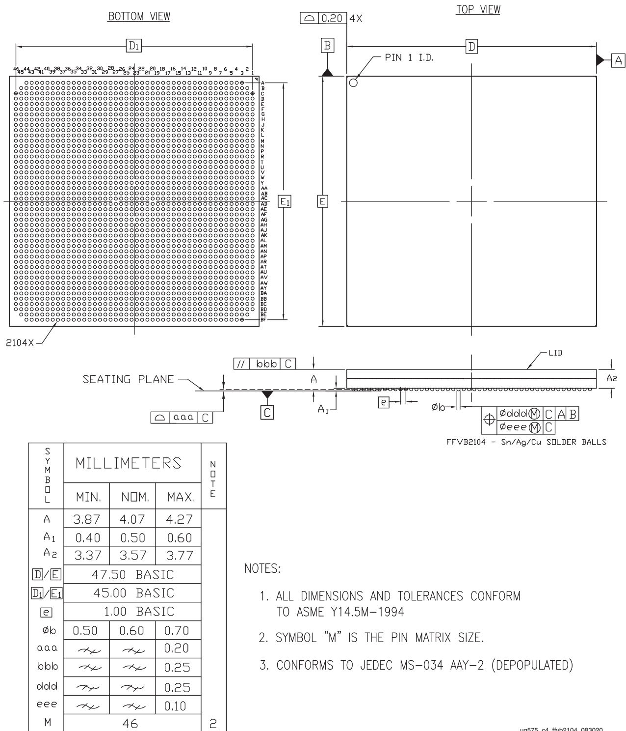
Figure 4-37: Package Dimensions for FFVB2104 (XCKU19P)
