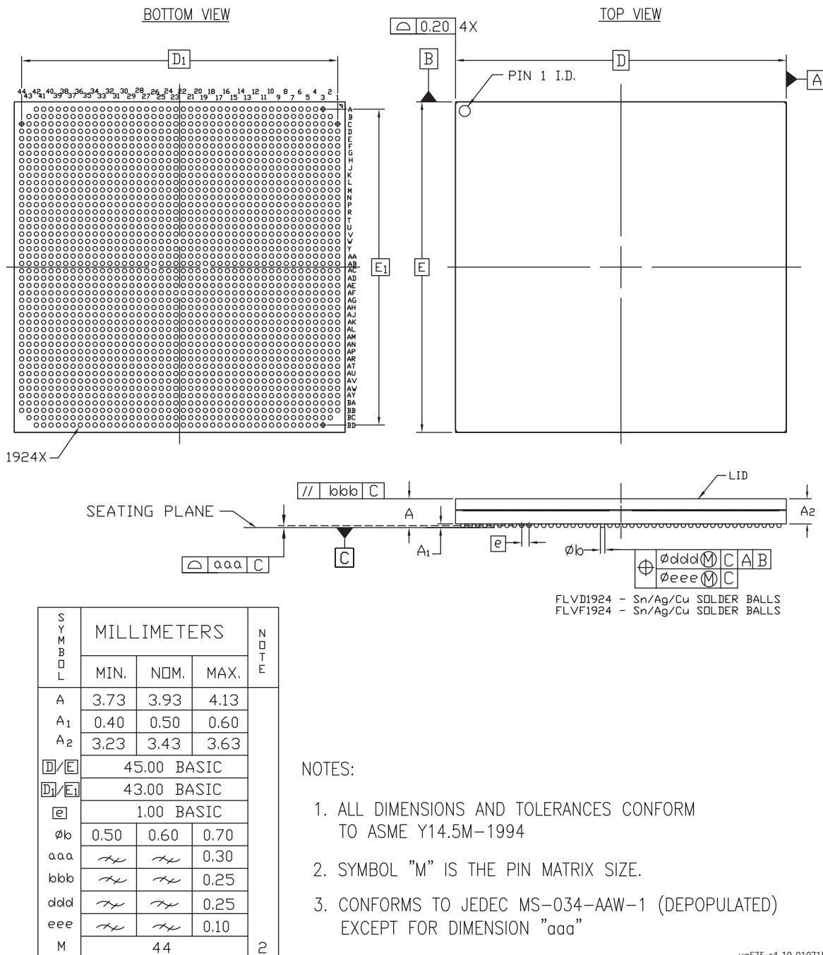
Figure 4-32: Package Dimensions for FLVD1924 (XCKU115) and FLVF1924 (XCKU085 and XCKU115)
