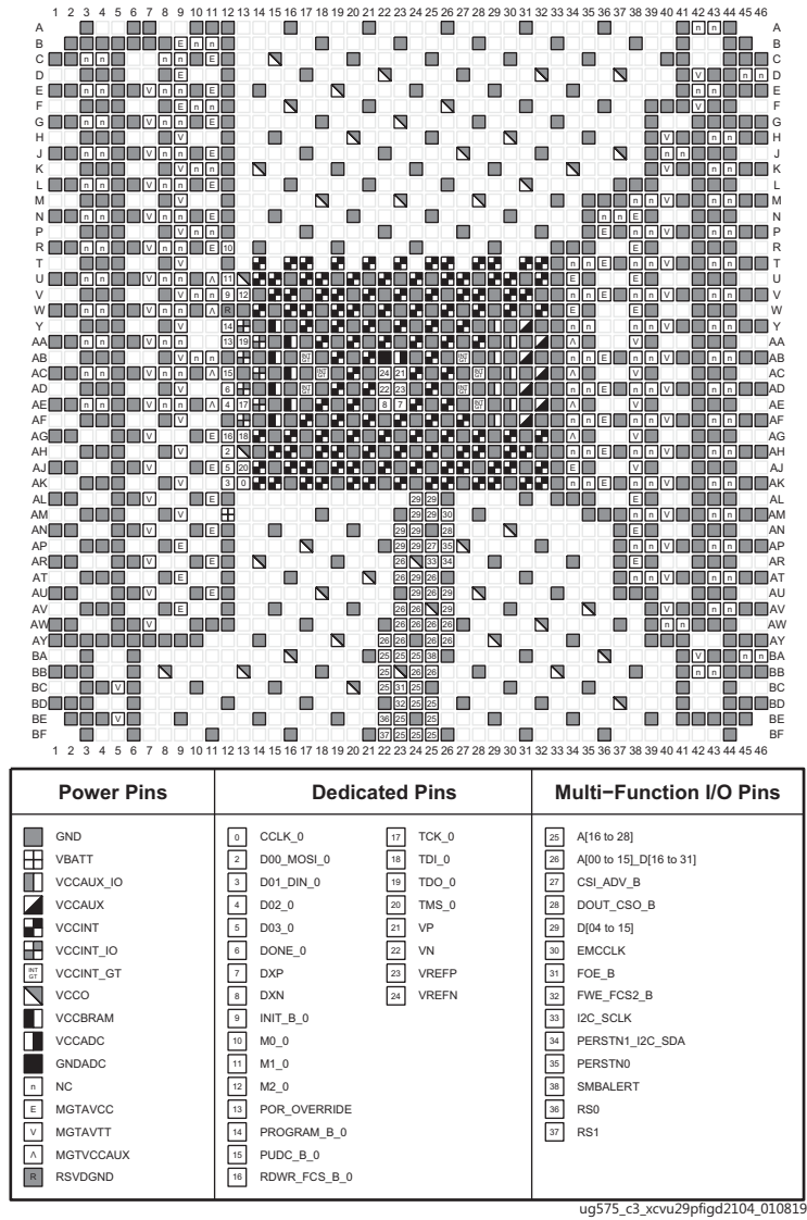
Figure 3-166: FIGD2104 Package—XCVU29P Configuration/Power Diagram
