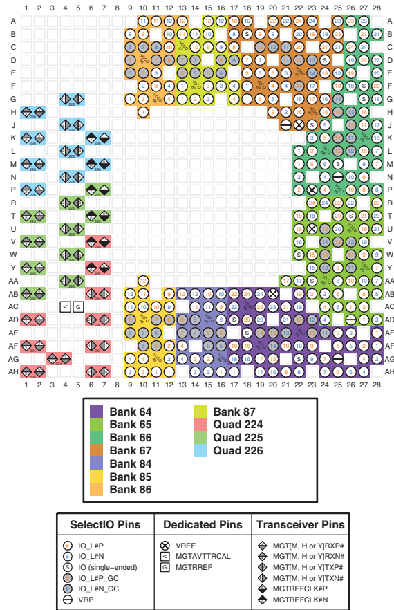
Figure 3-91: SFVB784 Package—XCAU25P I/O Bank Diagram
