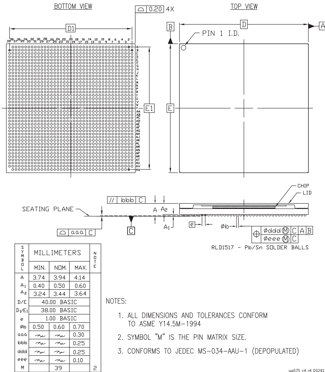
Figure 4-25: Package Dimensions for RLD1517 (XQKU115)
