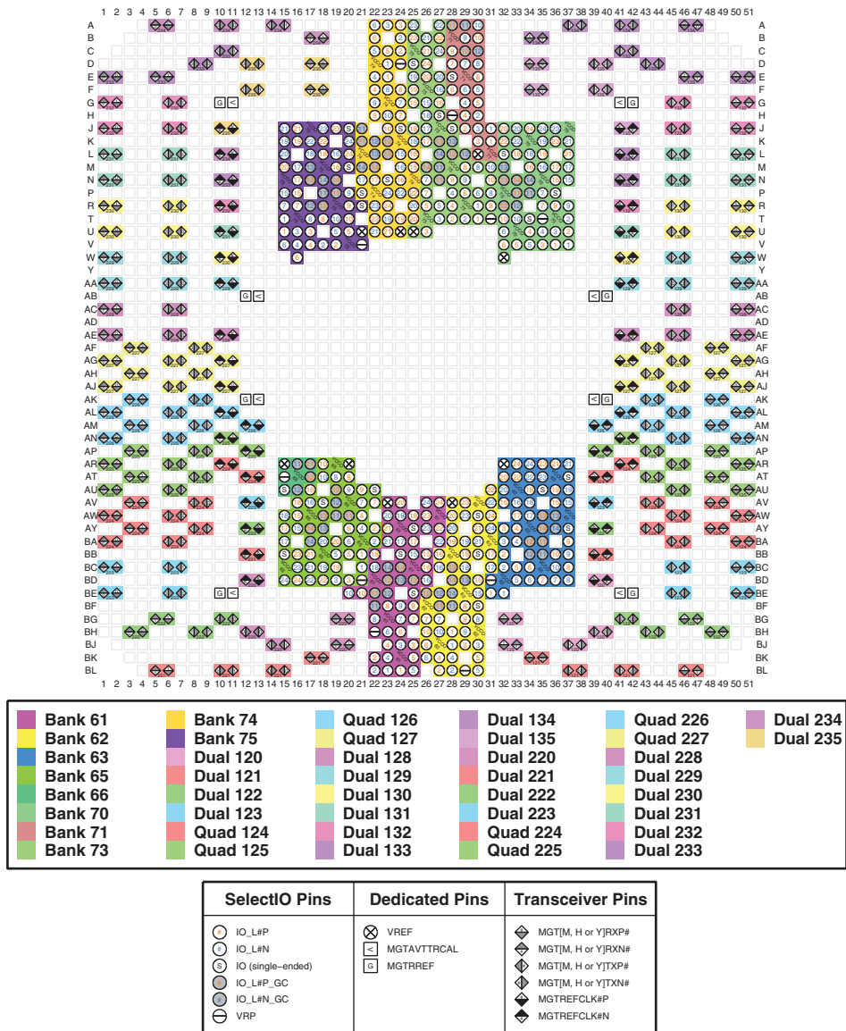
Figure 3-177: FSGA2577 Package—XCVU27P I/O Bank Diagram
