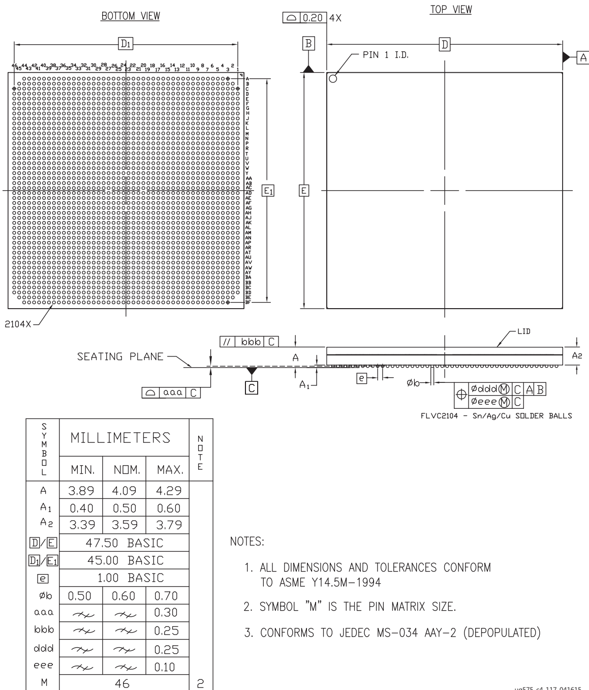
Figure 4-49: Package Dimensions for FLVC2104 (XCVU125)
