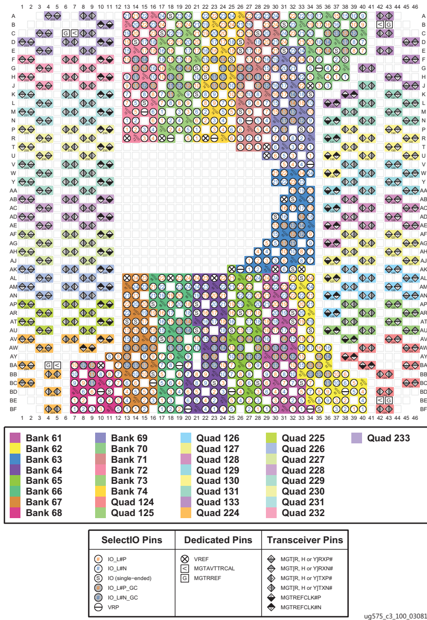
Figure 3-147: FHGB2104 Package—XCVU13P I/O Bank Diagram
