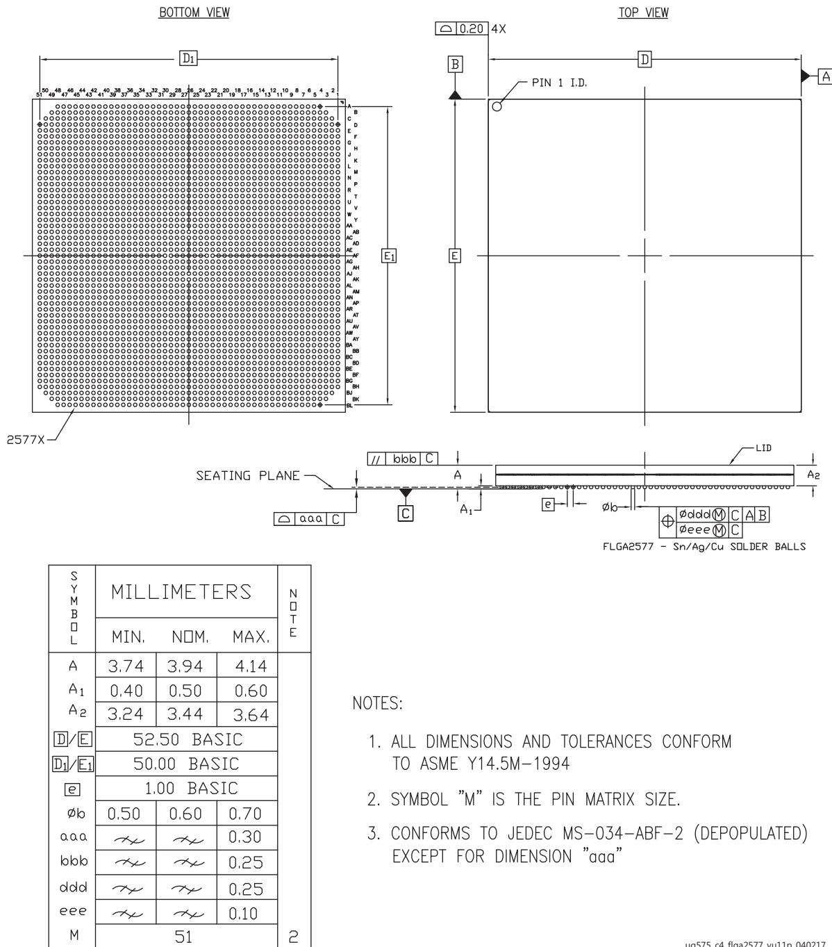
Figure 4-59: Package Dimensions for FLGA2577 (XCVU11P)
