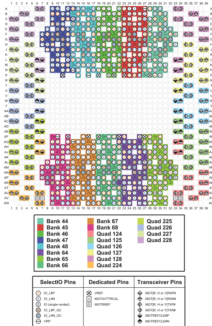
Figure 3-127: FFVC1517 Package—XCVU3P and FFRC1517 Package—XQVU3P I/O Bank Diagram
