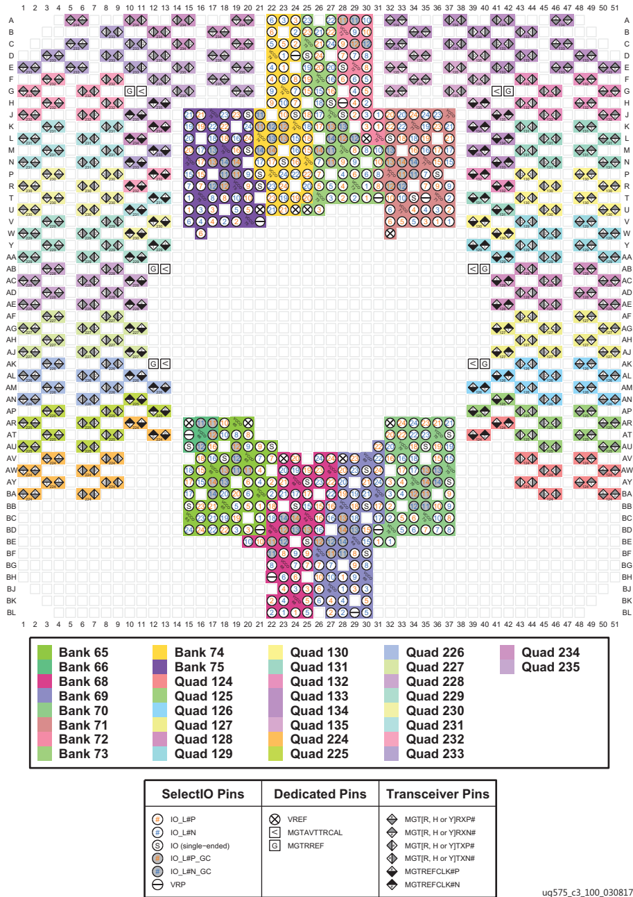
Figure 3-173: FLGA2577 Package—XCVU11P I/O Bank Diagram
