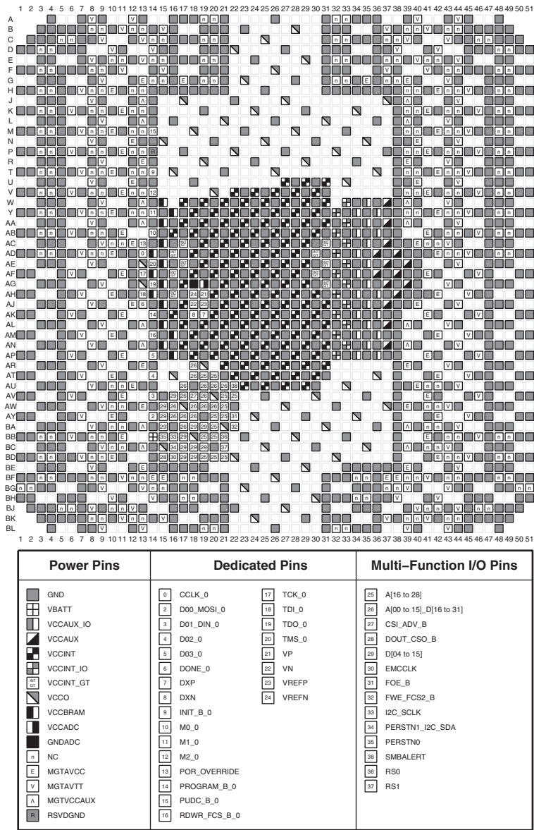
Figure 3-178: FSGA2577 Package—XCVU27P Configuration/Power Diagram
