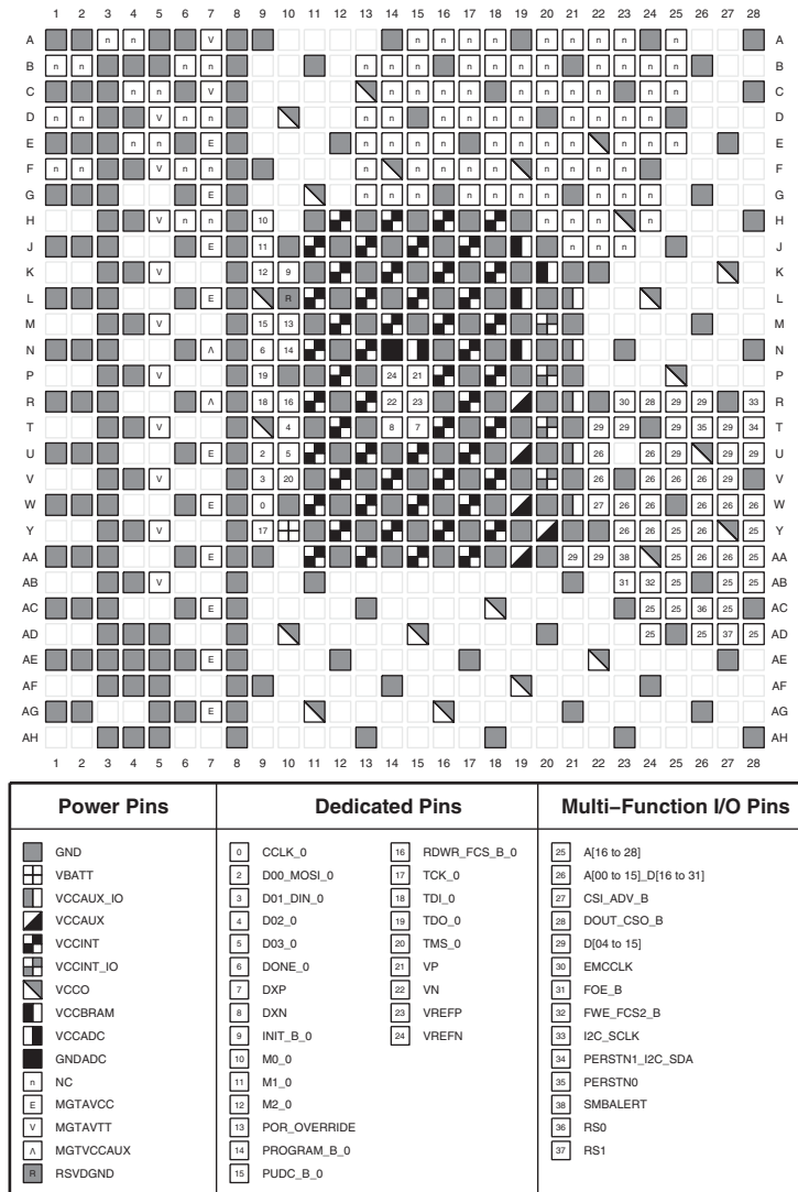
Figure 3-90: SFVB784 Package—XCAU20P Configuration/Power Diagram
