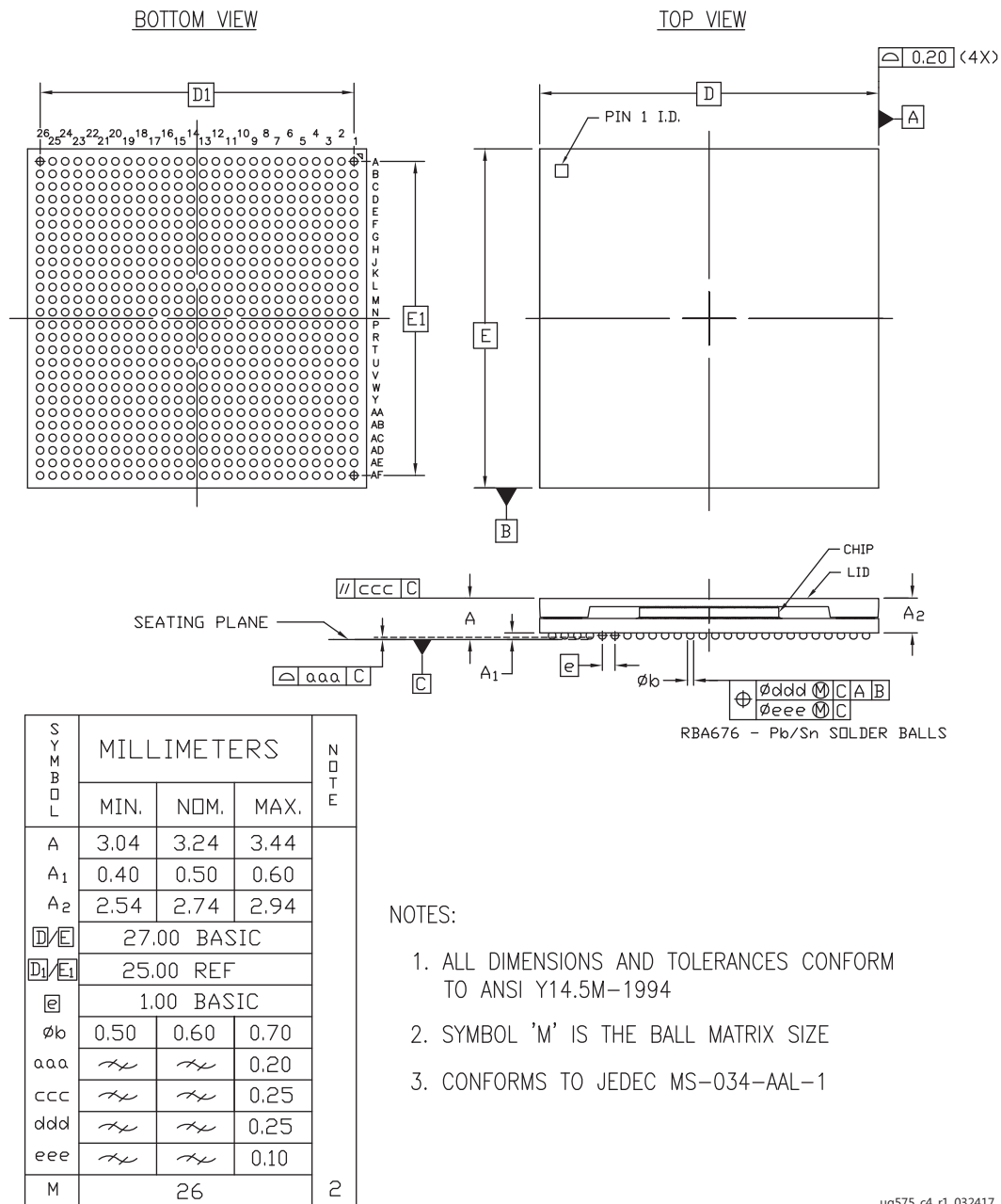
Figure 4-7: Package Dimensions for RBA676 (XQKU040)
