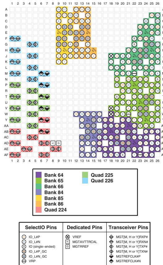
Figure 3-77: FFVB676 Package—XCAU10P I/O Bank Diagram
