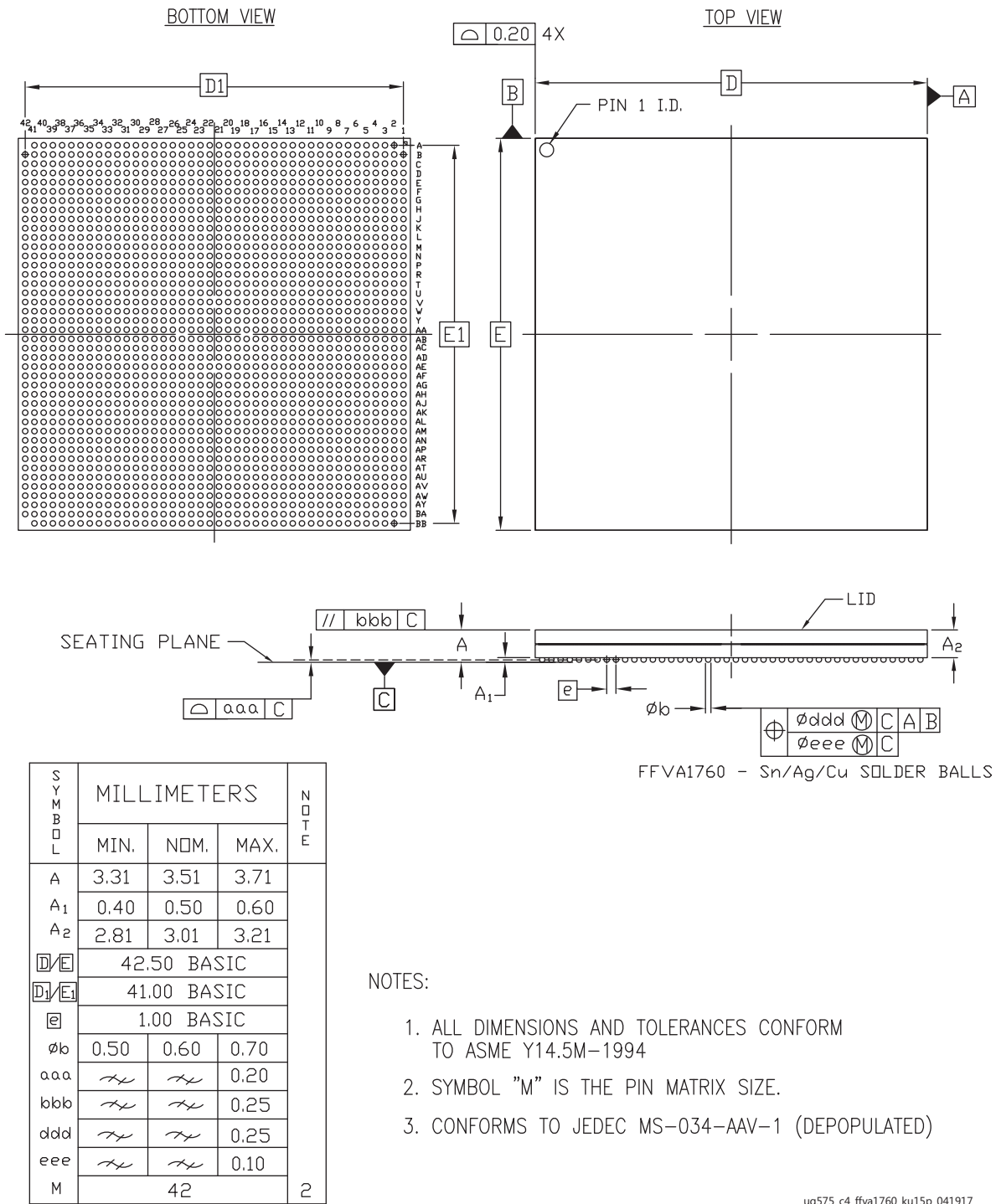
Figure 4-26: Package Dimensions for FFVA1760 (XCKU15P)
