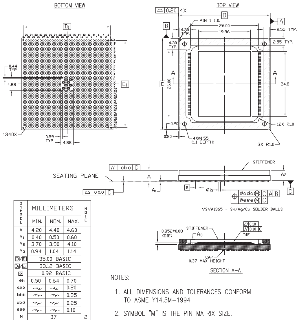
Figure 4-20: Package Dimensions for VSVA1365 (XCVU23P)
