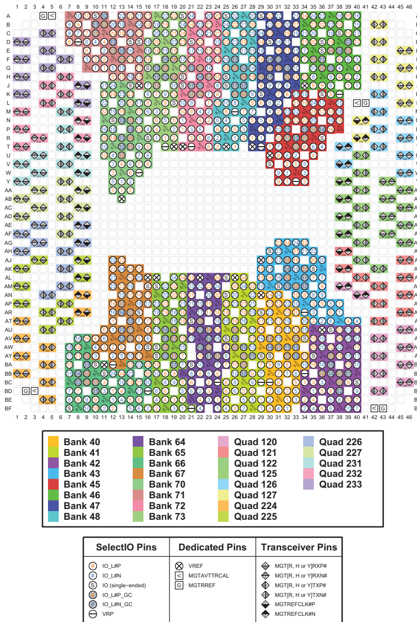
Figure 3-137: FLGA2104 Package—XCVU9P I/O Bank Diagram
