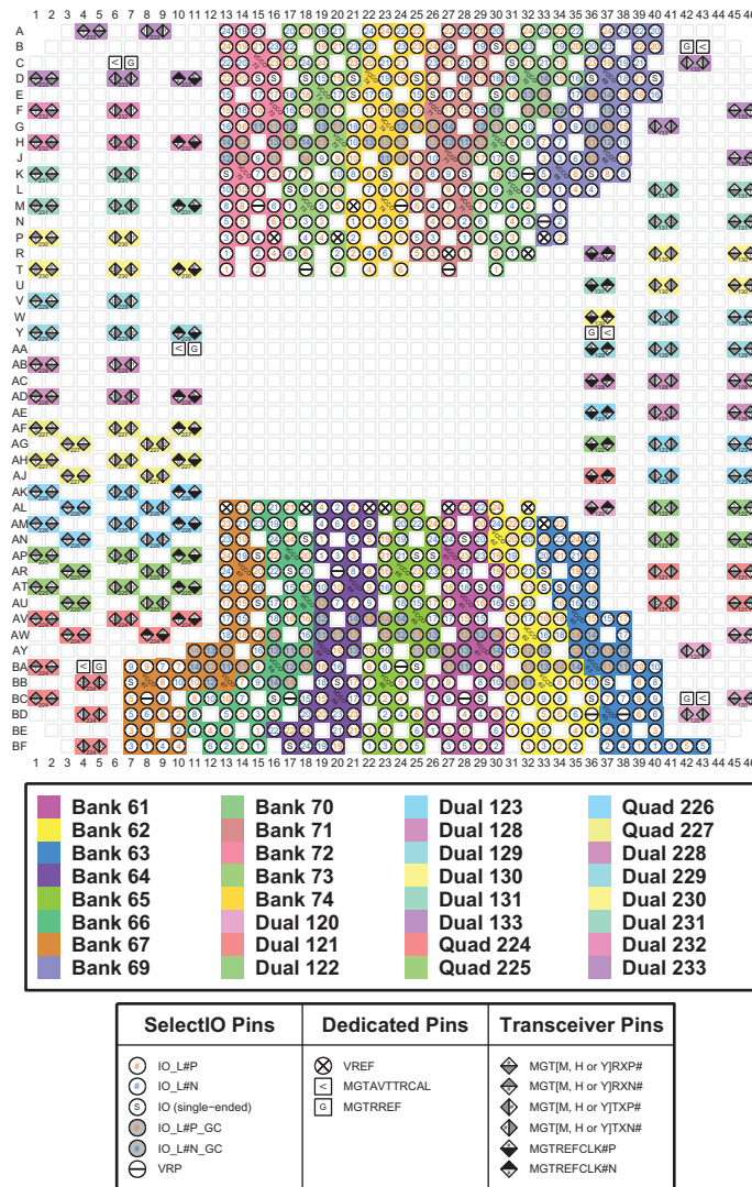
Figure 3-165: FIGD2104 Package—XCVU29P I/O Bank Diagram
