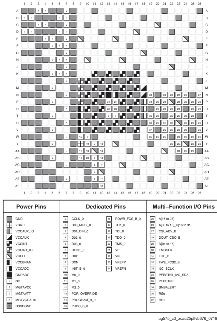
Figure 3-84: FFVB676 Package— XCAU25P Configuration/Power Diagram
