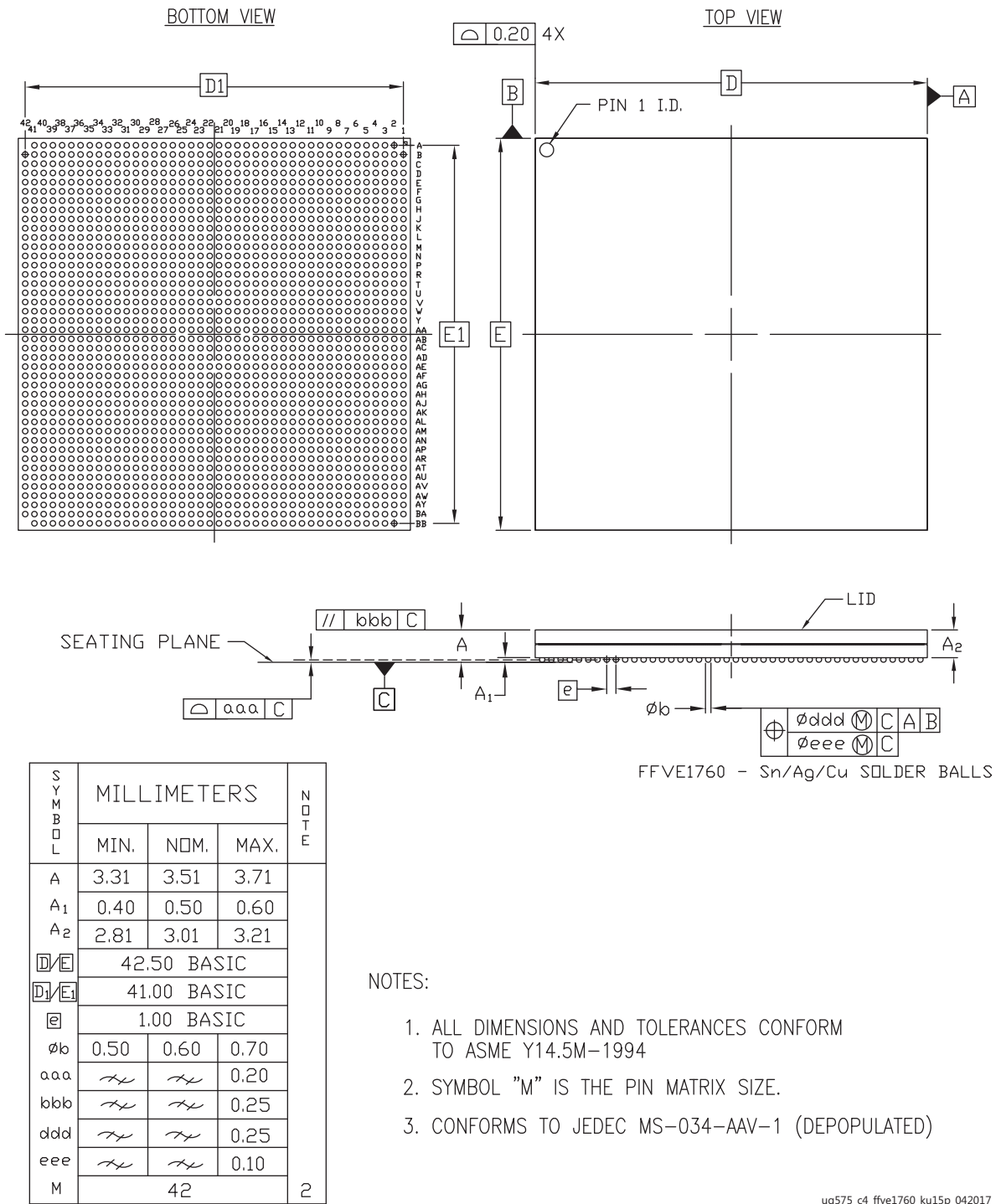
Figure 4-29: Package Dimensions for FFVE1760 (XCKU15P)
