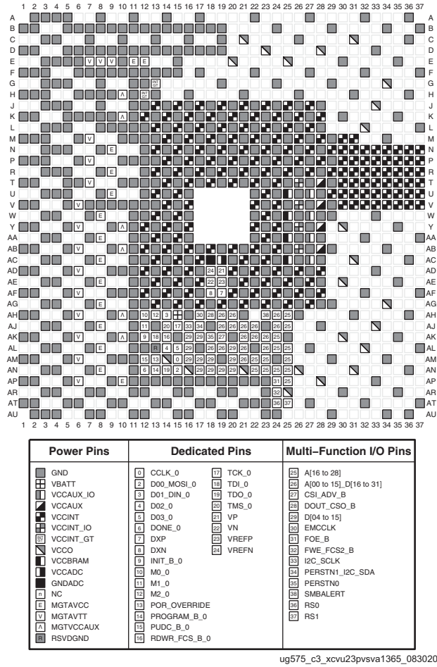
Figure 3-193: VSVA1365 Package—XCVU23P Configuration/Power Diagram
