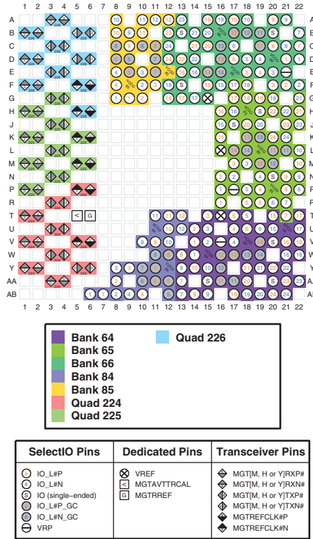
Figure 3-87: SBVB484 Package—XCAU15P I/O Bank Diagram
