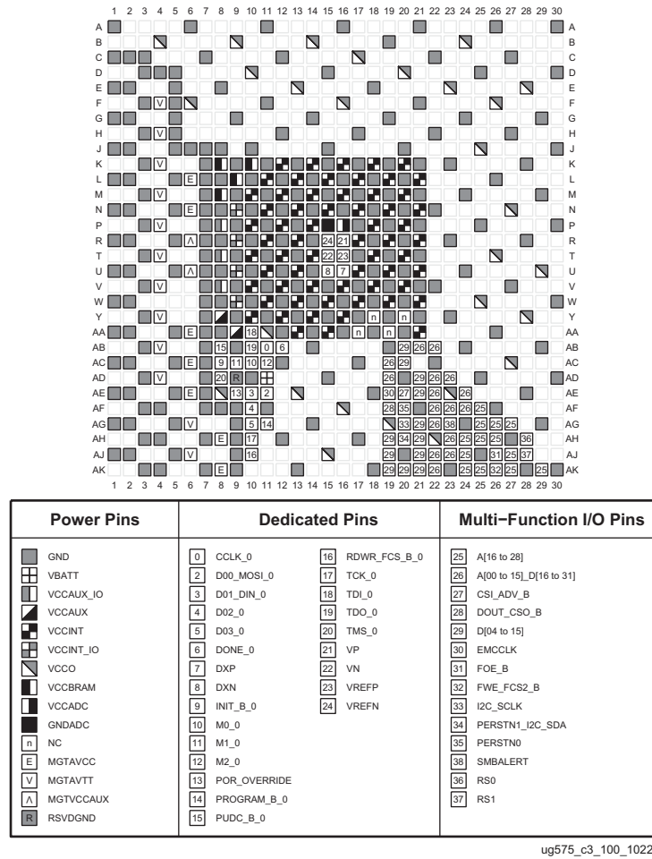
Figure 3-106: FFVD900 Package—XCKU11P Configuration/Power Diagram
