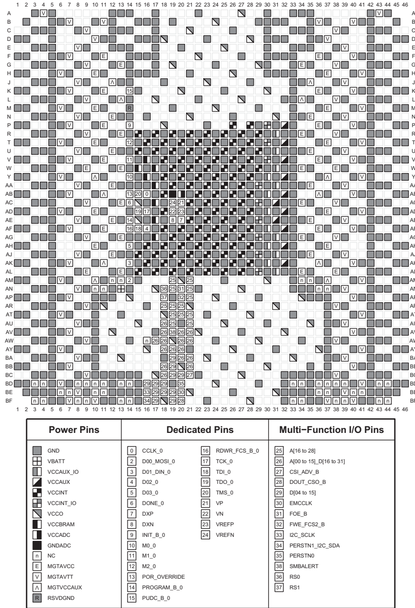
Figure 3-154: FLGC2104 Package—XCVCU11P and FLRC2104 Package—XQVCU11P Configuration/Power Diagram
