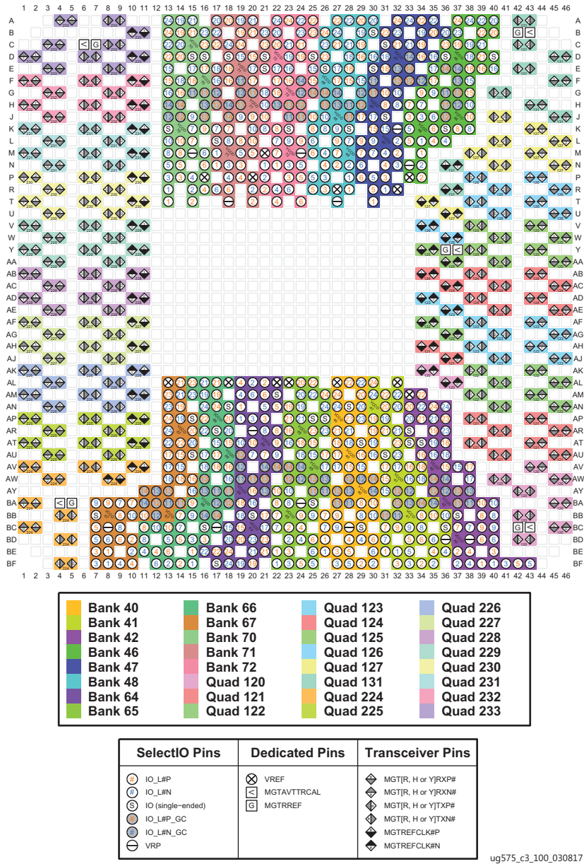
Figure 3-157: FSGD2104 Package—XCVU9P I/O Bank Diagram
