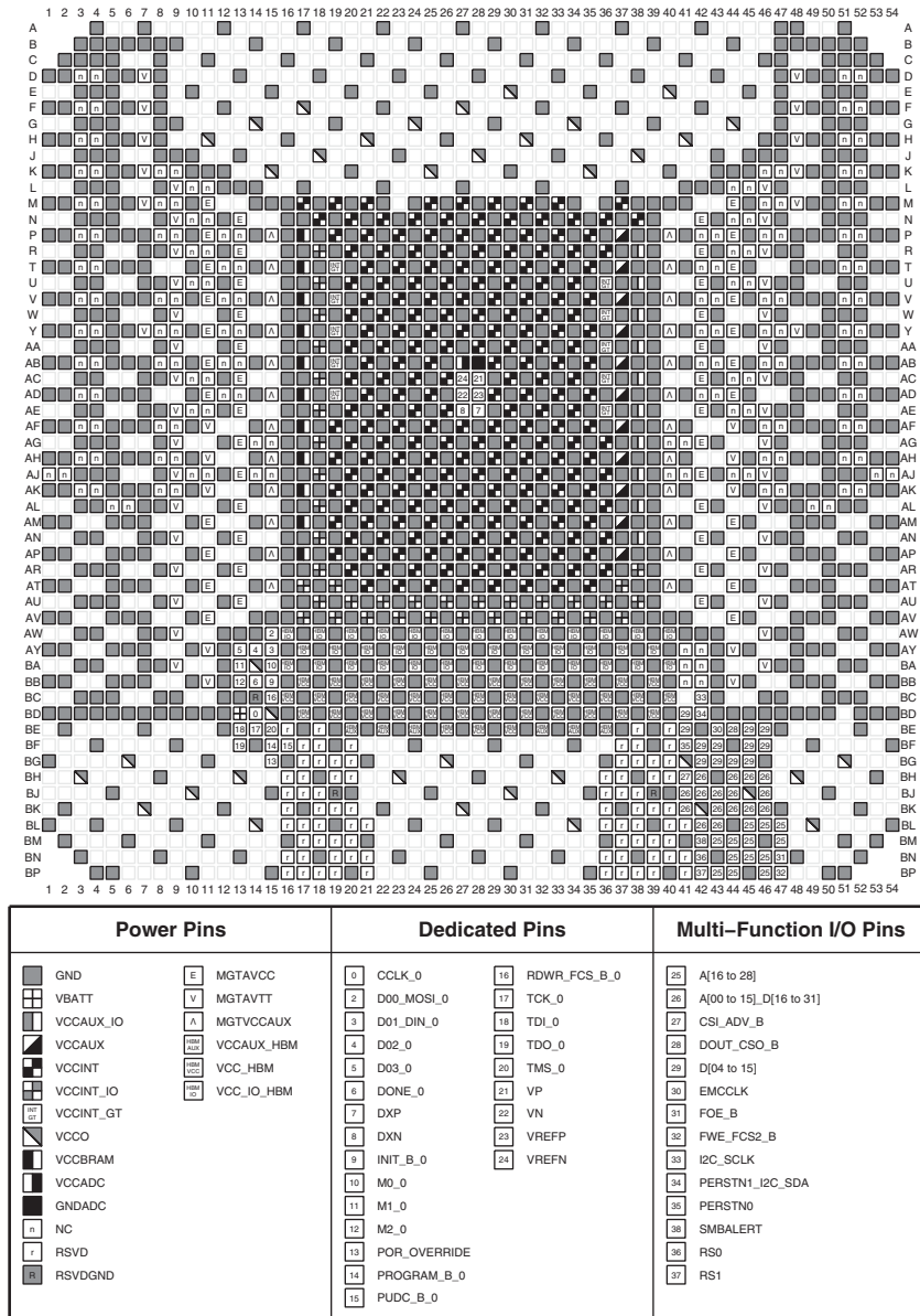
Figure 3-186: FSVK2892 Package—XCVU57P Configuration/Power Diagram
