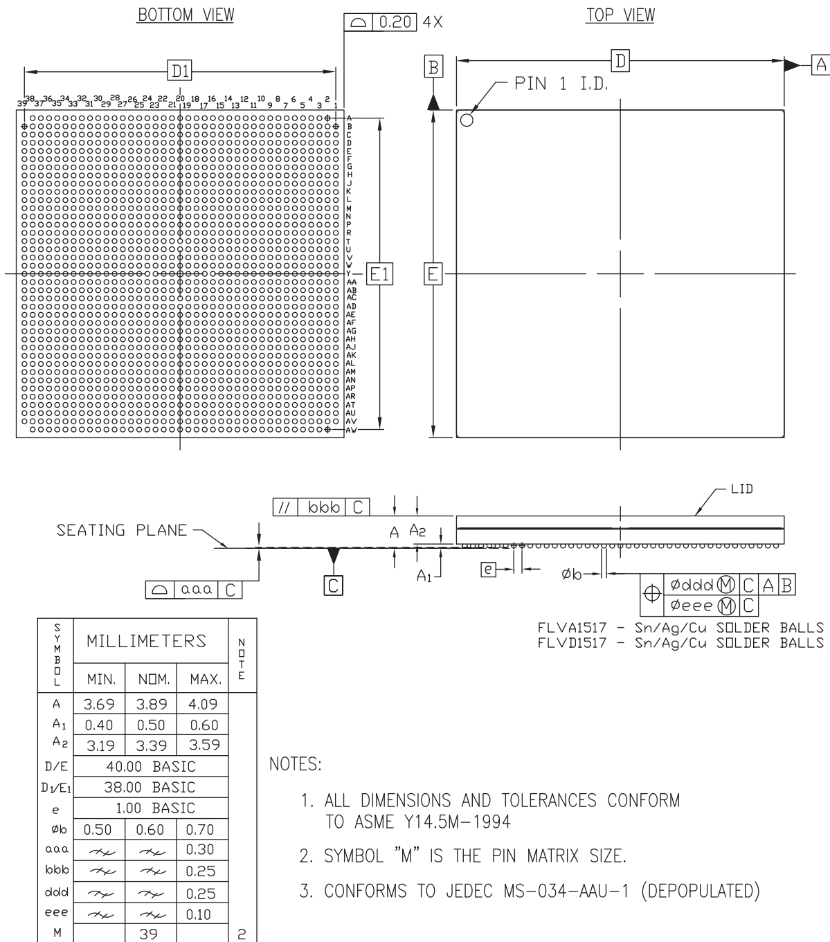
Figure 4-24: Package Dimensions for FLVA1517 (XCKU085 and XCKU115) and FLVD1517 (XCKU115 and XCVU125)
