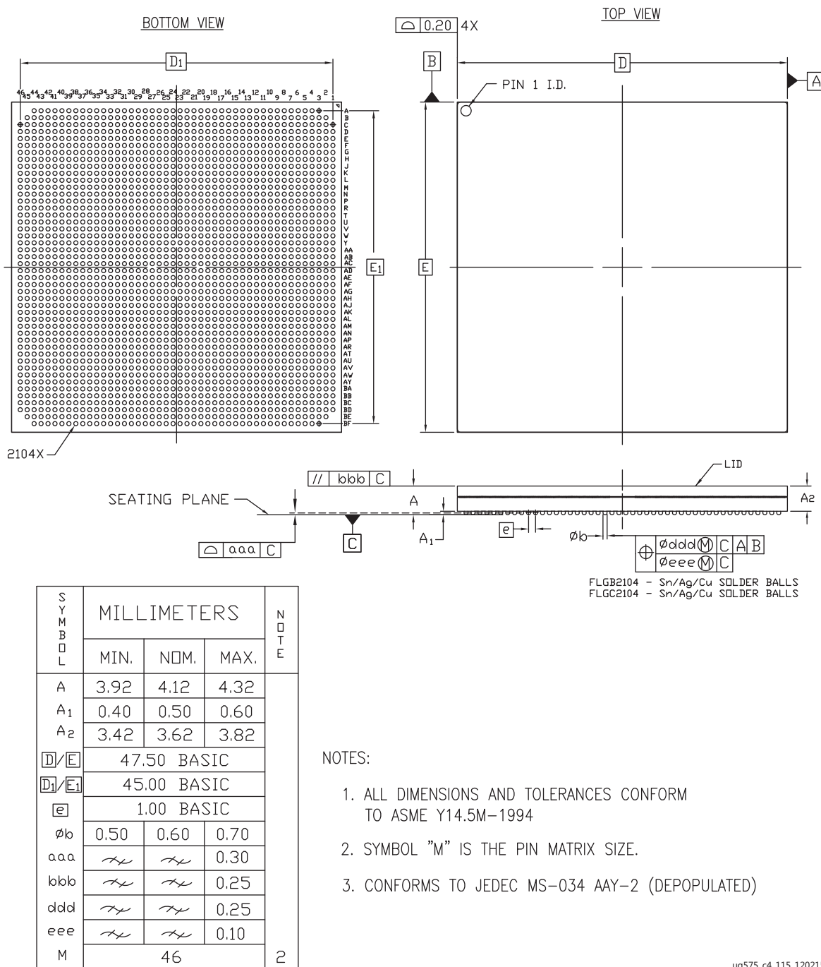
Figure 4-44: Package Dimensions for FLGB2104 (XCVU160 and XCVU190) and FLGC2104 (XCVU160 and XCVU190)
