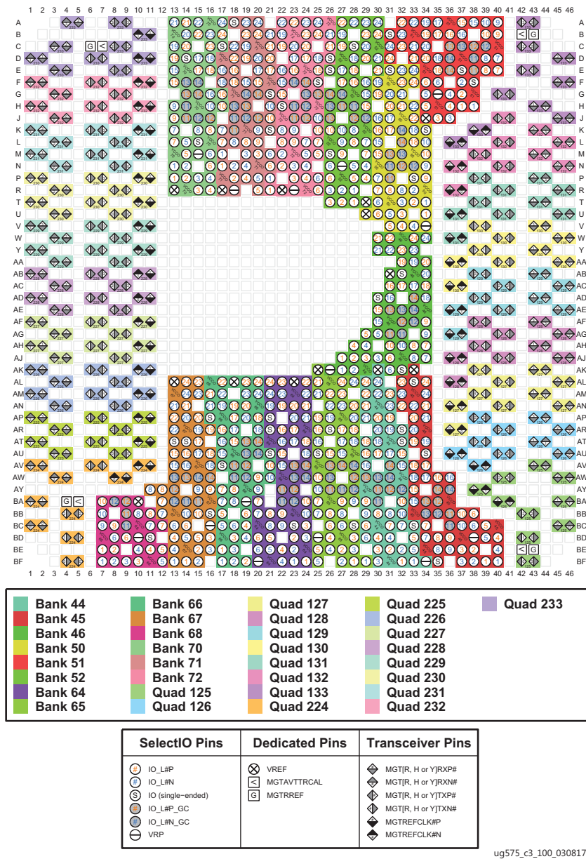
Figure 3-141: FLVB2104 Package—XCVU5P and XCVU7P and FLRB2104 Package—XQVU7P I/O Bank Diagram
