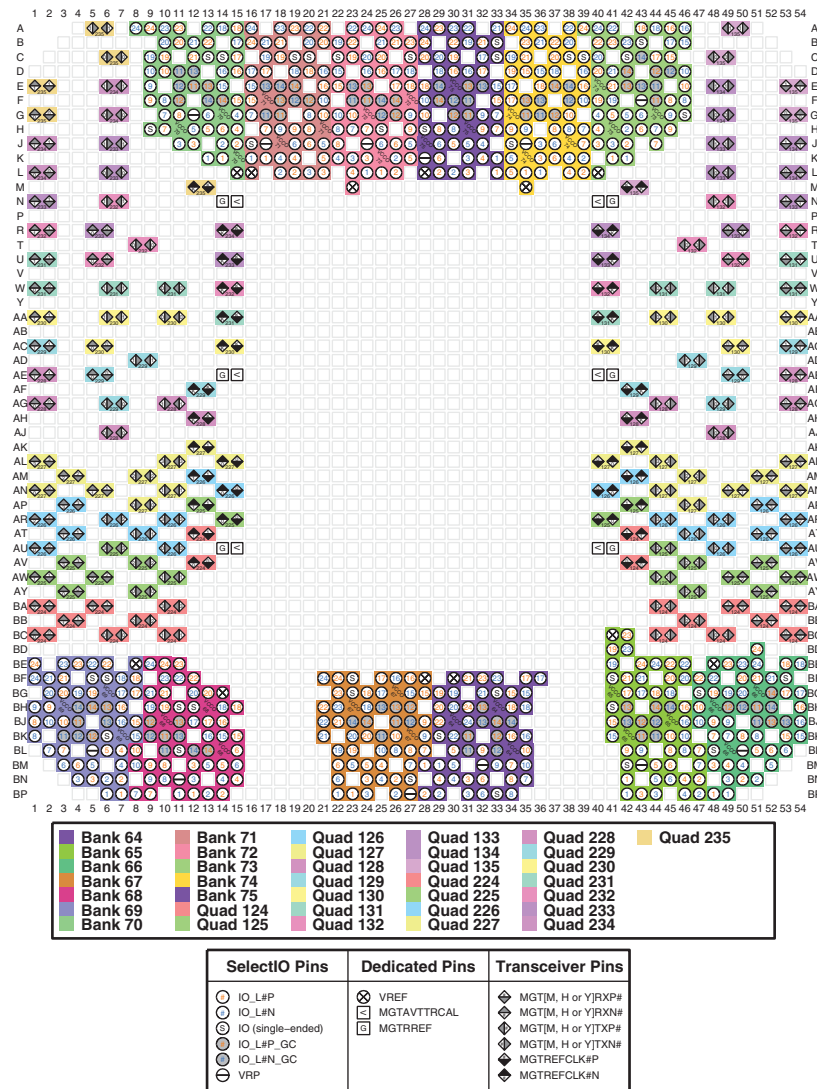
Figure 3-185: FSVK2892 Package—XCVU57P I/O Bank Diagram
