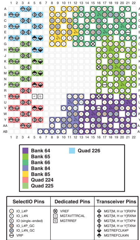
Figure 3-85: SBVB484 Package—XCAU10P I/O Bank Diagram
