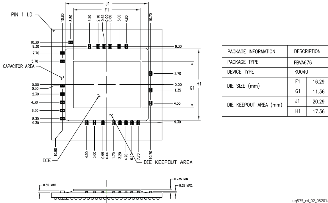
Figure 4-4: FBVA676 Package (XCKU035 and XCKU040) Die Dimensions with Capacitor Locations
