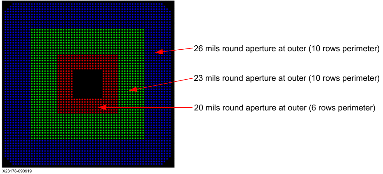
Figure 8-4: Bull's Eye Stencil Aperture
