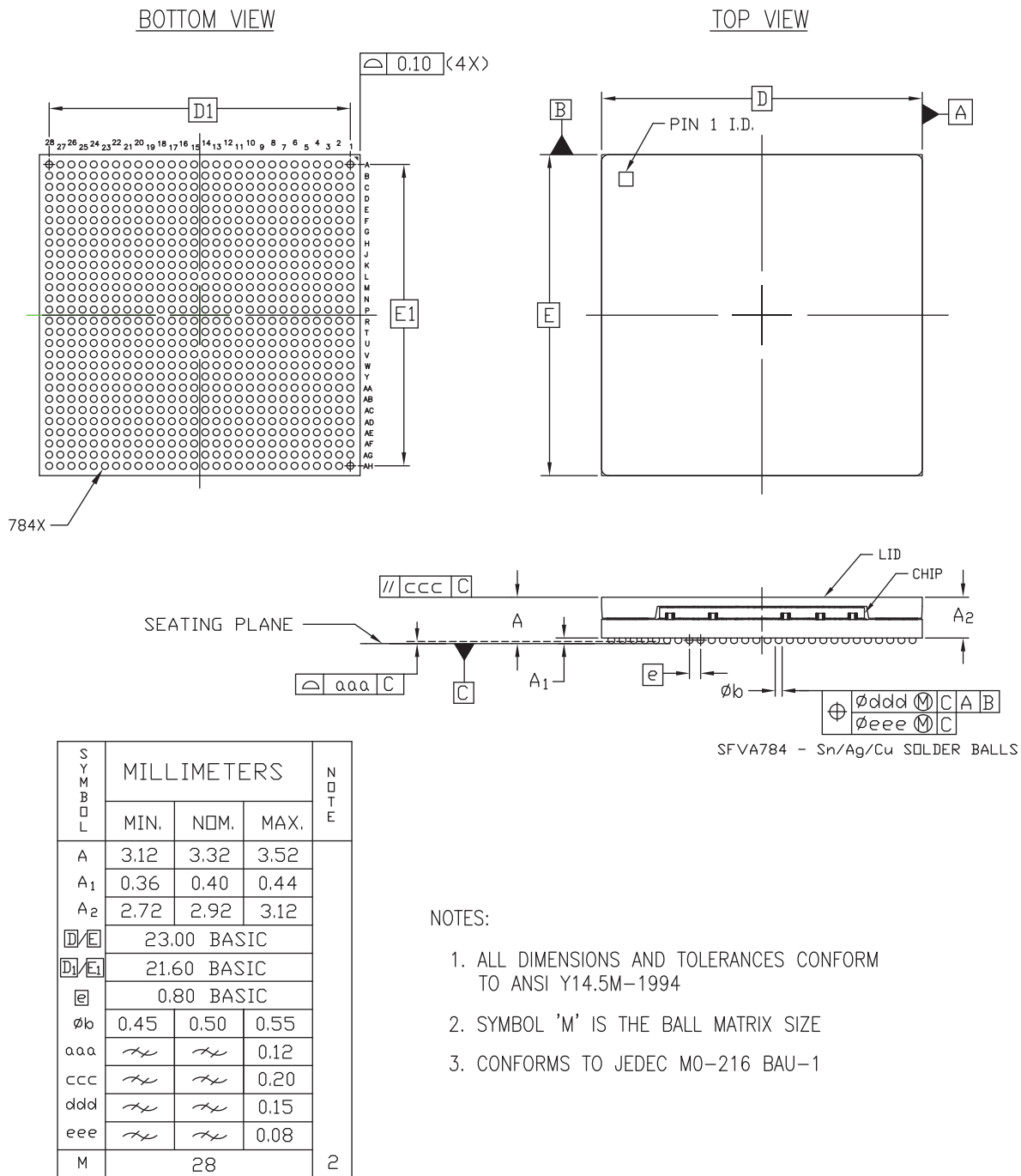
Figure 4-8: Package Dimensions for SFVA784 (XCKU035 and XCKU040)
