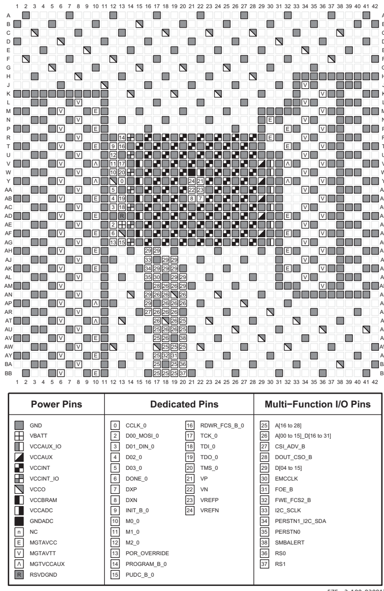
Figure 3-121: FFVE1760 Package—XCKU15P Configuration/Power Diagram
