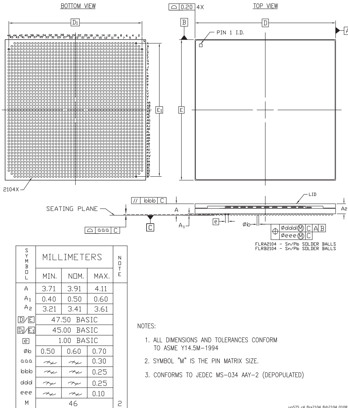
Figure 4-42: Package Dimensions for FLRA2104 (XQVU7P) and FLRB2104 (XQVU7P)
