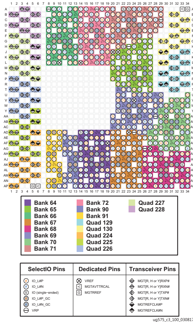
Figure 3-113: FFVA1156 Package—XCKU15P and FFRA1156 Package—XQKU15P I/O Bank Diagram
