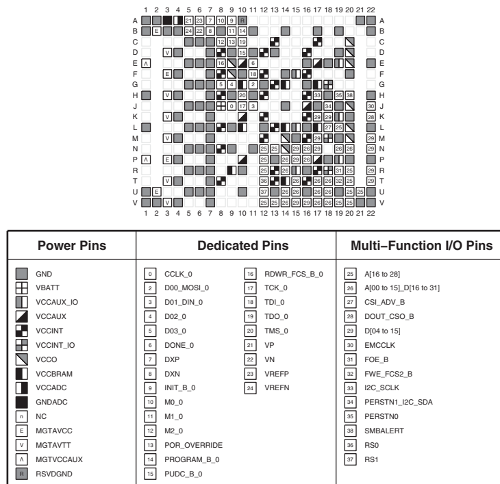
Figure 3-96: UBVA368 Package—XCAU15P Configuration/Power Diagram
