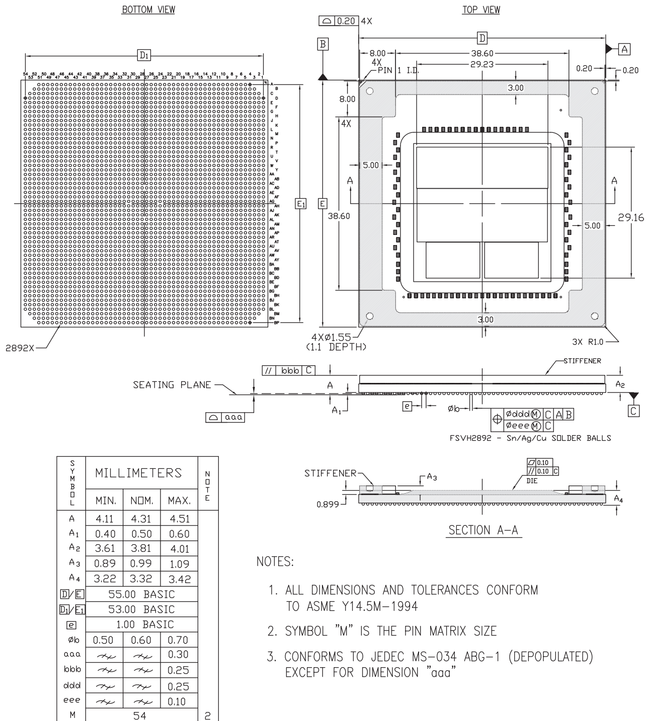
Figure 4-62: Package Dimensions for FSVH2892 (XCVU35P and XCVU45P)
