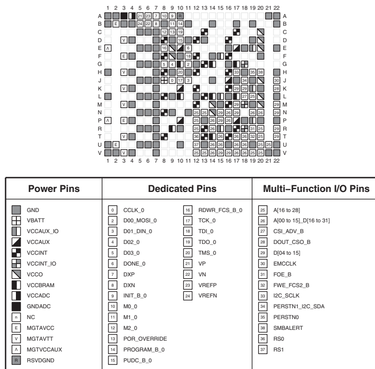
Figure 3-94: UBVA368 Package—XCAU10P Configuration/Power Diagram
