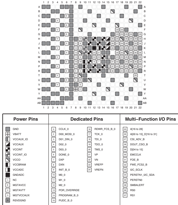
Figure 3-86: SBVB484 Package— XCAU10P Configuration/Power Diagram
