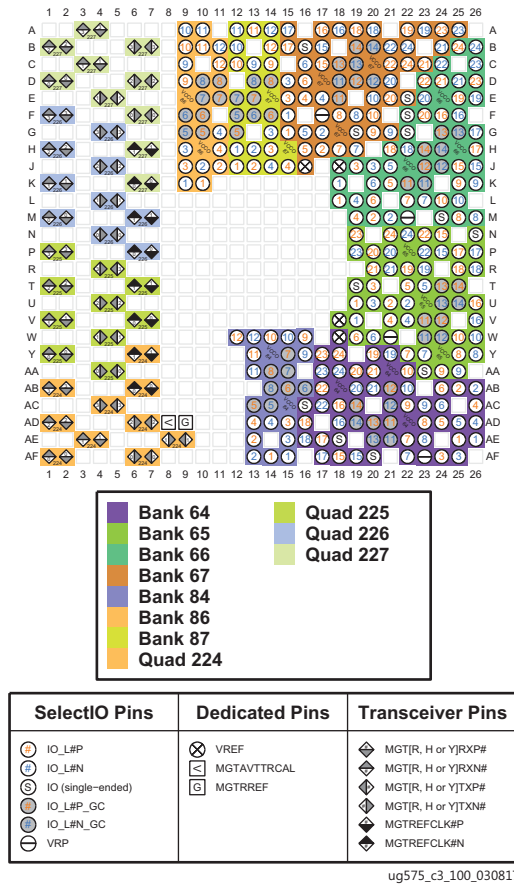
Figure 3-99: FFVB676 Package—XCKU3P and XCKU5P and FFRB676 Package—XQKU5P I/O Bank Diagram
