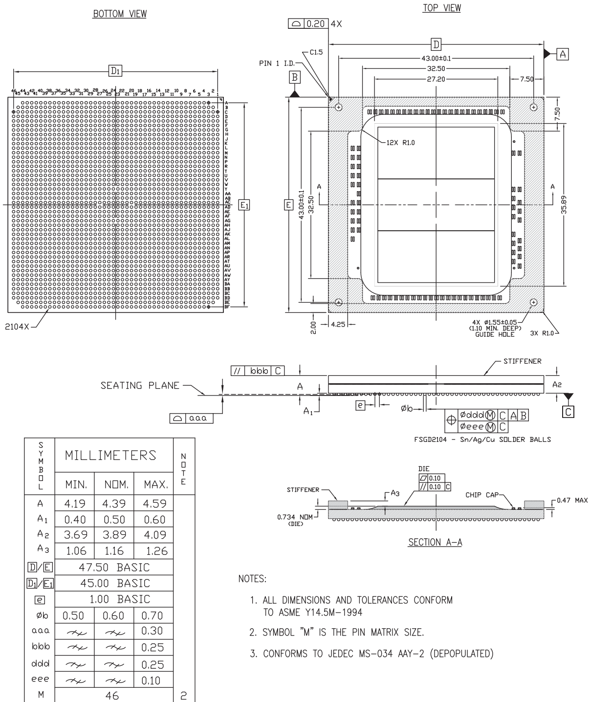
Figure 4-52: Package Dimensions for FSGD2104 (XCVU9P)
