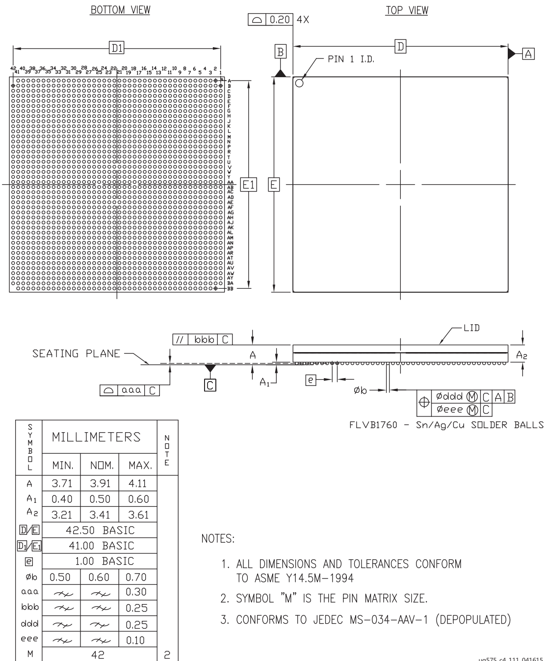
Figure 4-28: Package Dimensions for FLVB1760 (XCKU085, XCKU115, and XCVU125)
