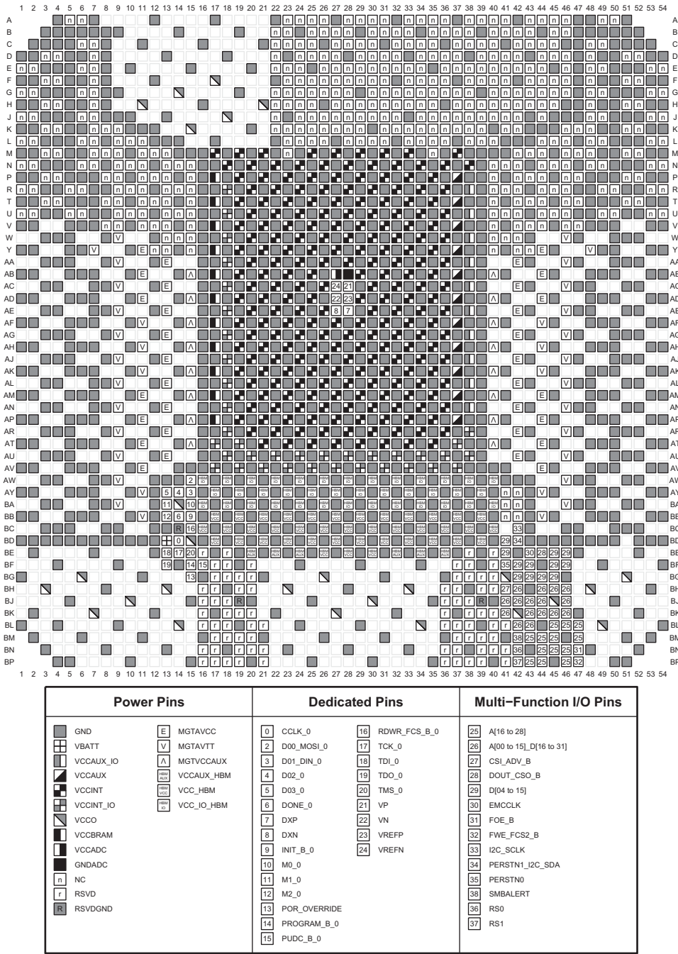
Figure 3-182: FSVH2892 Package—XCVU35P and XCVU45P Configuration/Power Diagram
