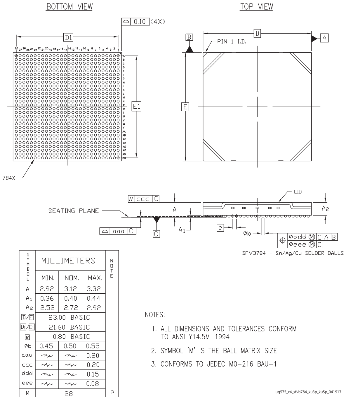
Figure 4-9: Package Dimensions for SFVB784 (XCAU20P, XCAU25P, XCKU3P, and XCKU5P)
