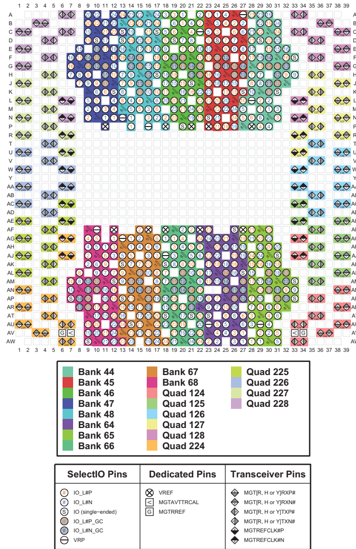
Figure 3-126: FFVC1517 Package—XCVU3P and FFRC1517 Package—XQVU3P I/O Bank Diagram
