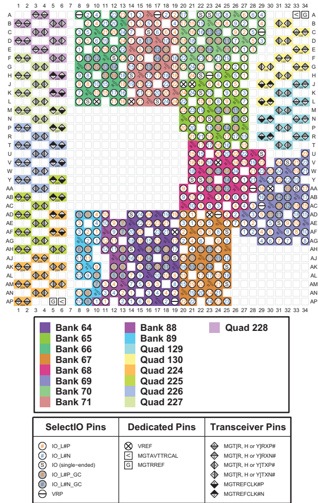
Figure 3-111: FFVA1156 Package—XCKU11P I/O Bank Diagram
