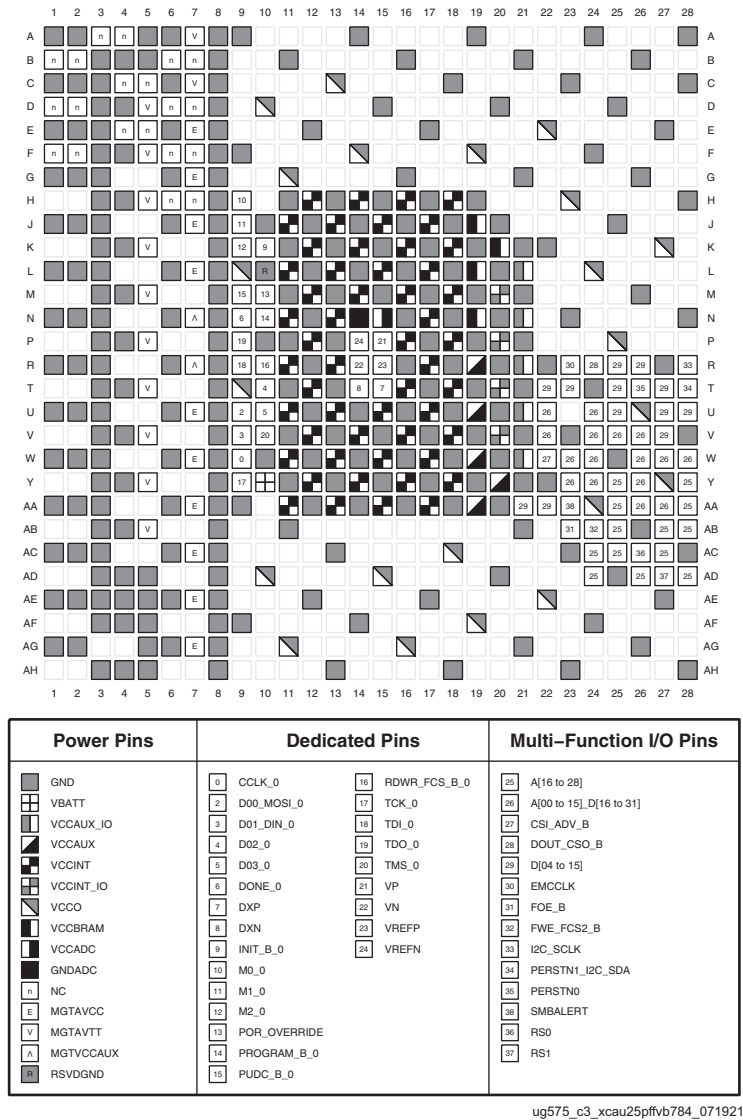
Figure 3-92: SFVB784 Package—XCAU25P Configuration/Power Diagram
