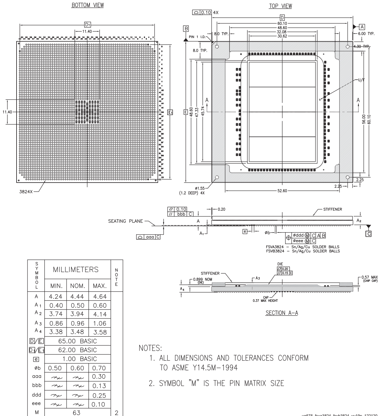
Figure 4-65: Package Dimensions for FSVA3824 and FSVB3824 (XCVU19P)
