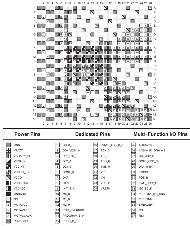
Figure 3-98: FFVA676 Package—XCKU3P and XCKU5P Configuration/Power Diagram
