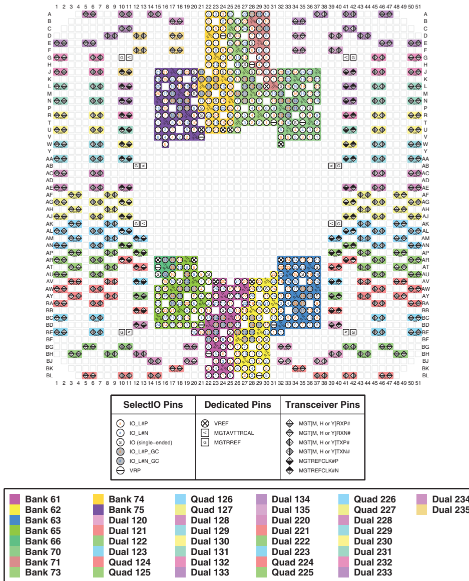
Figure 3-179: FSGA2577 Package—XCVU29P I/O Bank Diagram
