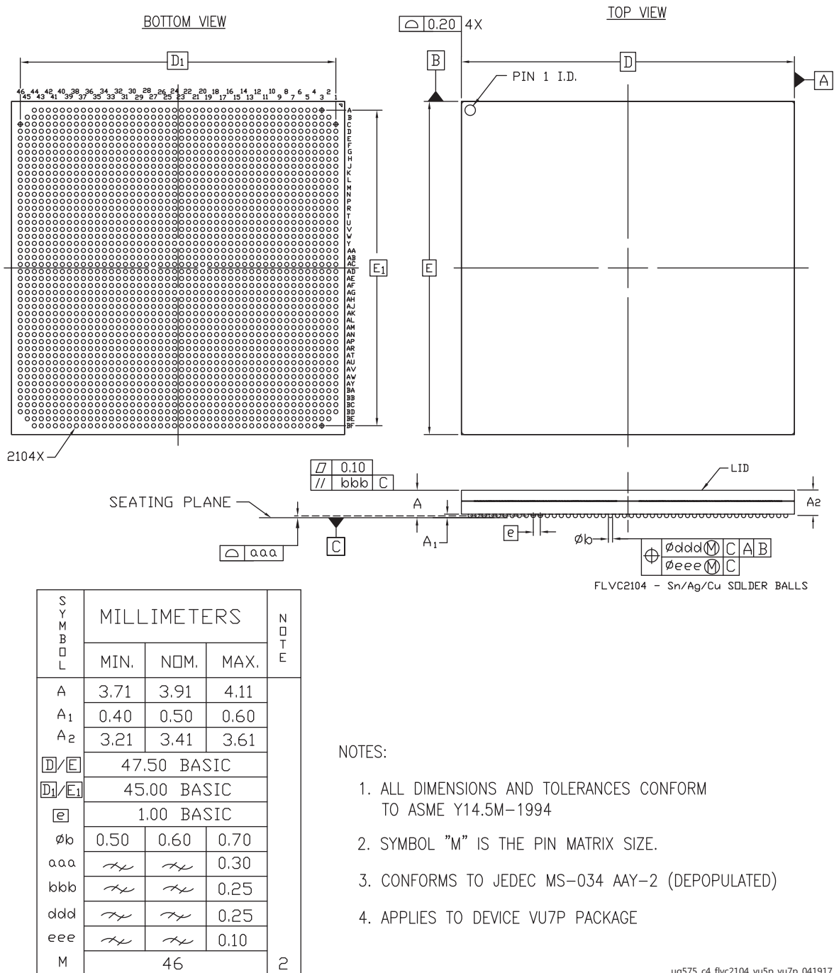
Figure 4-50: Package Dimensions for FLVC2104 (XCVU5P and XCVU7P)
