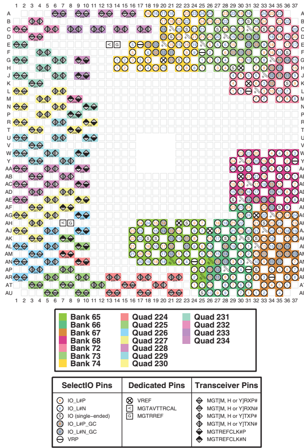
Figure 3-192: VSVA1365 Package—XCVU23P I/O Bank Diagram
