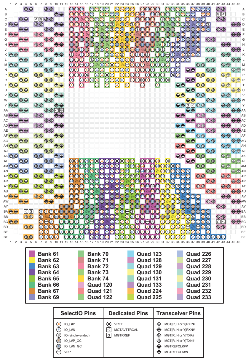
Figure 3-161: FIGD2104 Package—XCVU13P I/O Bank Diagram
