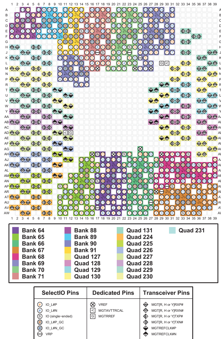
Figure 3-115: FFVE1517 Package—XCKU11P I/O Bank Diagram
