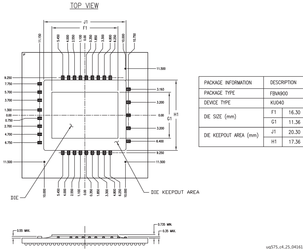
Figure 4-12: FBVA900 Package (XCKU035 and XCKU040) Die Dimensions with Capacitor Locations
