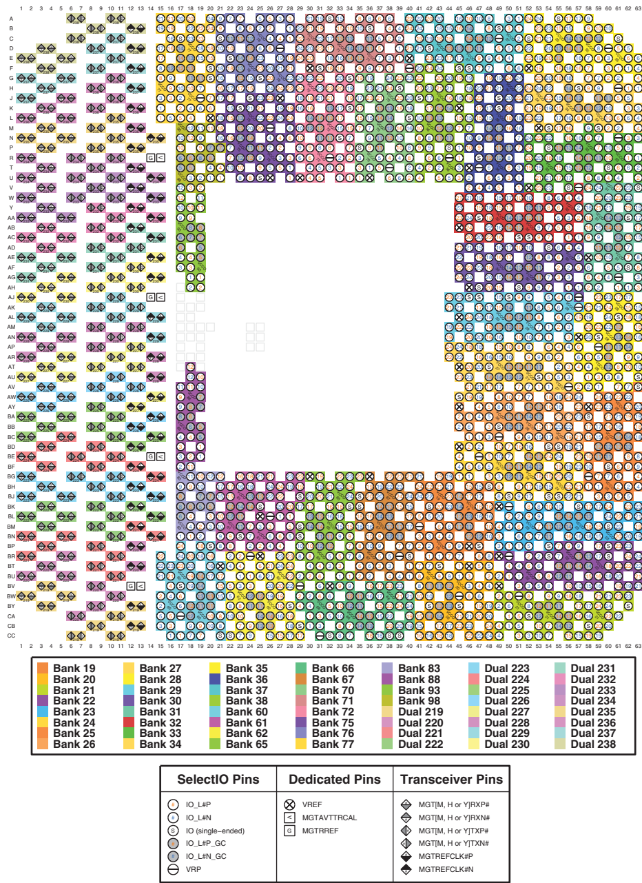
Figure 3-190: FSVB3824 Package—XCVU19P I/O Bank Diagram
