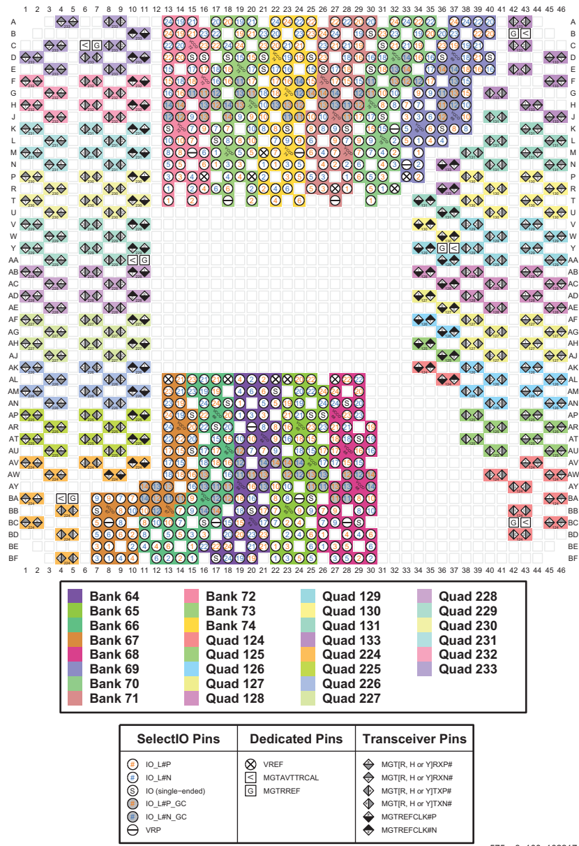
Figure 3-159: FSGD2104 Package—XCVU11P I/O Bank Diagram
