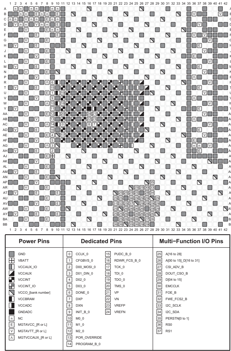
Figure 3-52: FFVB1760 Package—XCVU080 and XCVU095 Configuration/Power Diagram
