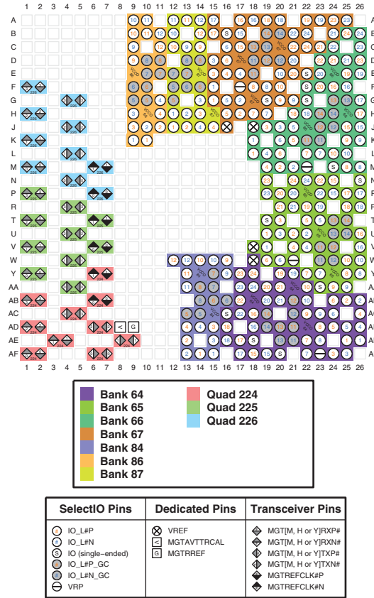
Figure 3-83: FFVB676 Package—XCAU25P I/O Bank Diagram
