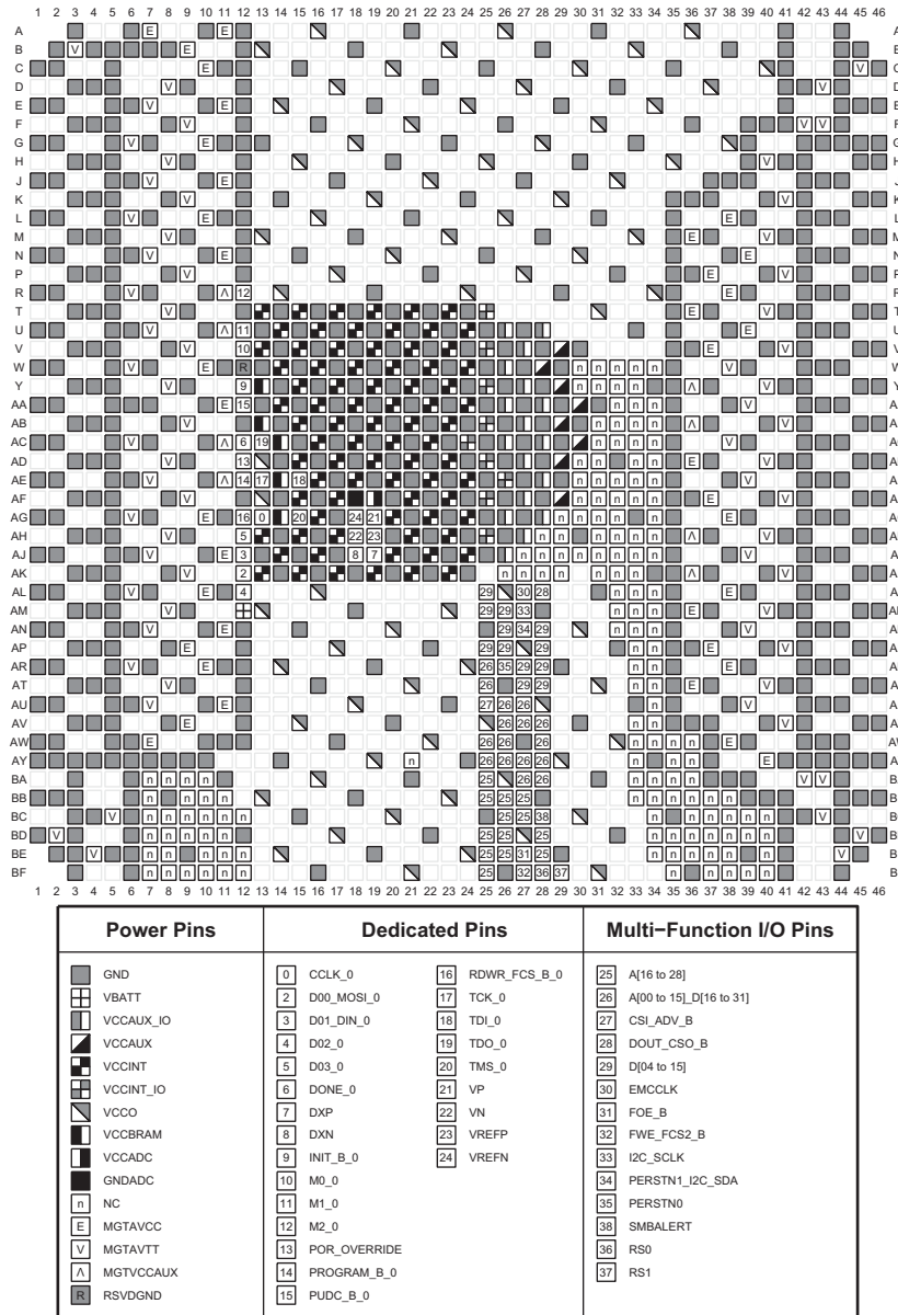
Figure 3-146: FLGB2104 Package—XCVU11P Configuration/Power Diagram
