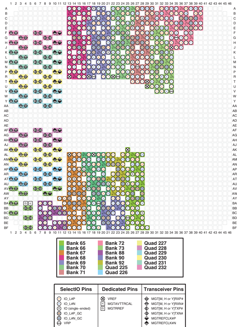
Figure 3-124: FFVB2104 Package—XCKU19P I/O Bank Diagram
