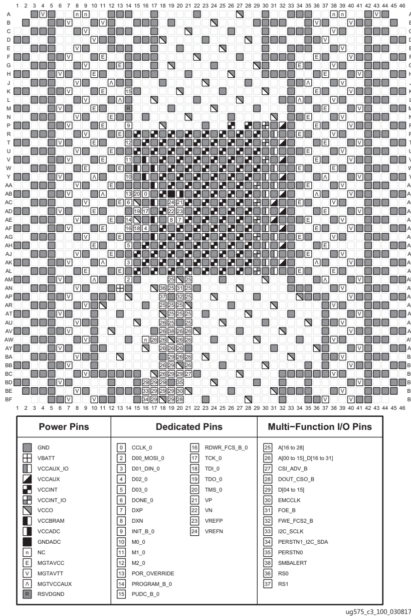
Figure 3-152: FLGC2104 Package—XCVU9P Configuration/Power Diagram
