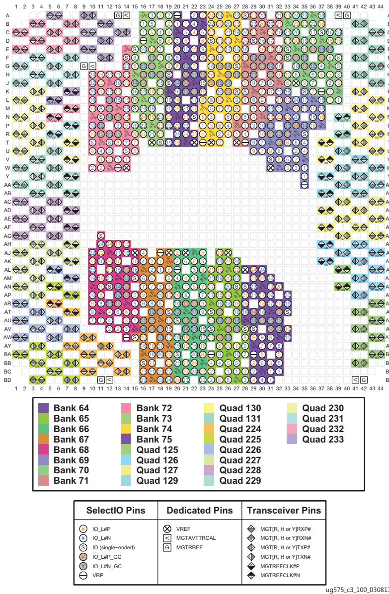
Figure 3-131: FLGF1924 Package—XCVU11P I/O Bank Diagram
